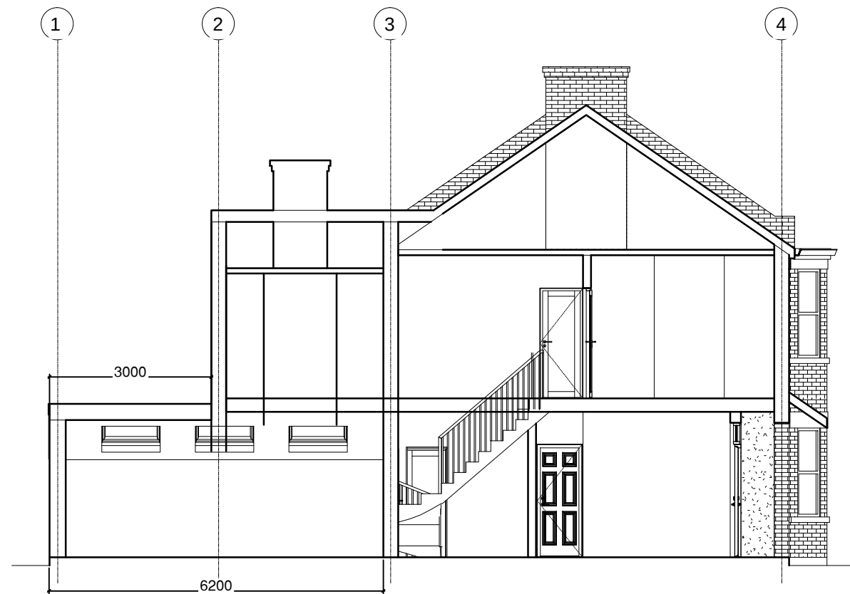
PROPOSED SECTION
