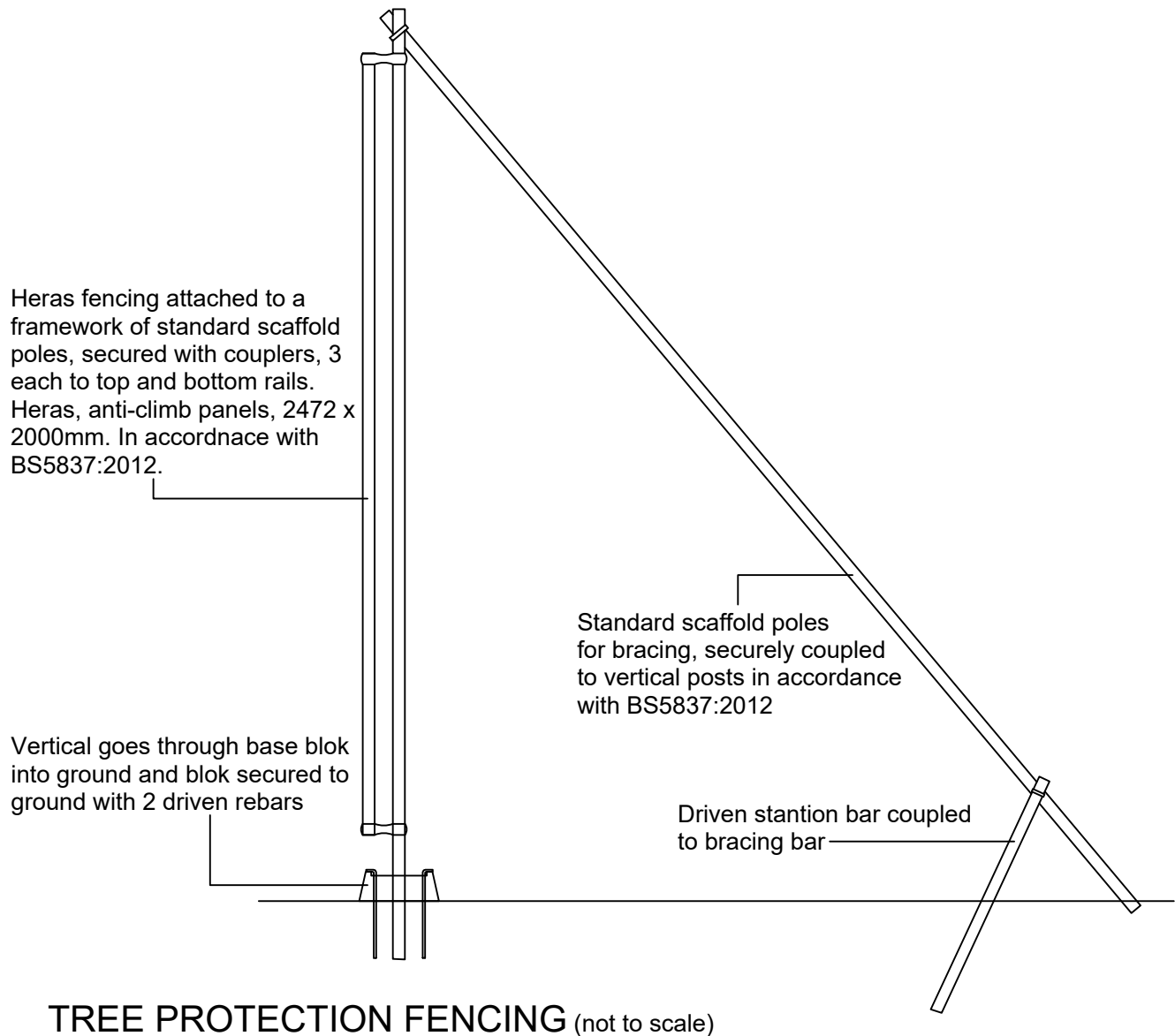
TREE PROTECTION FENCING (not to scale)
