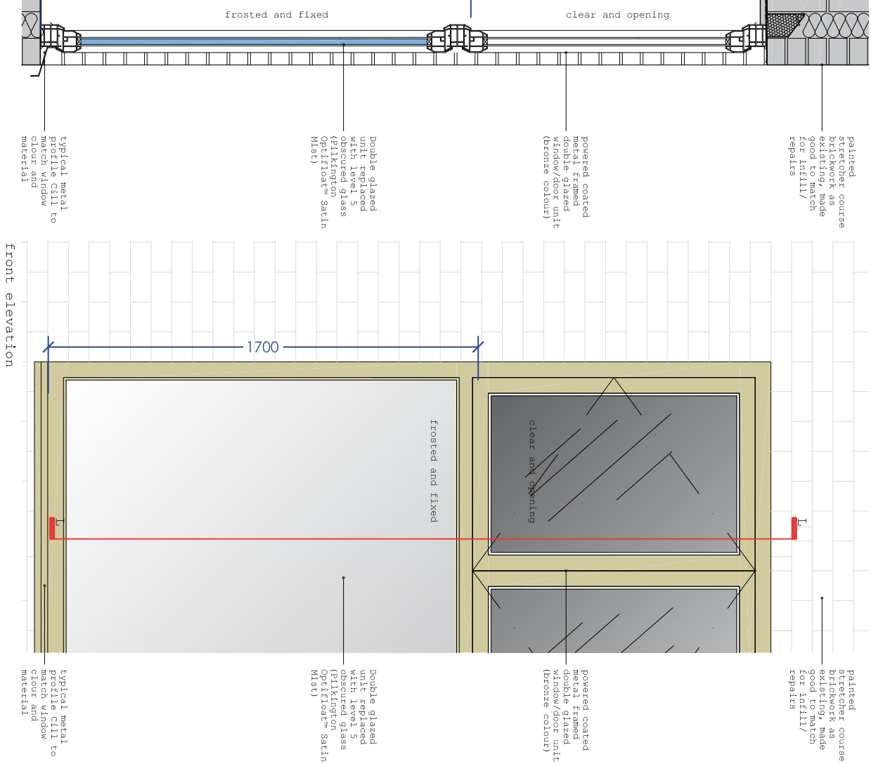
typical section and elevation
