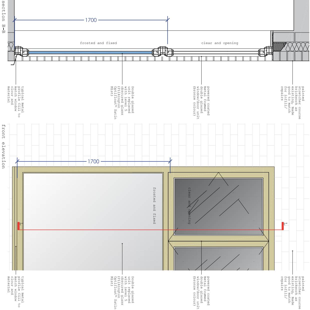
typical section and elevation
