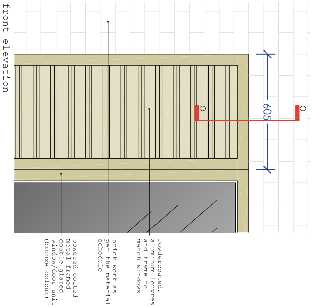
DETAIL O - louvered window
