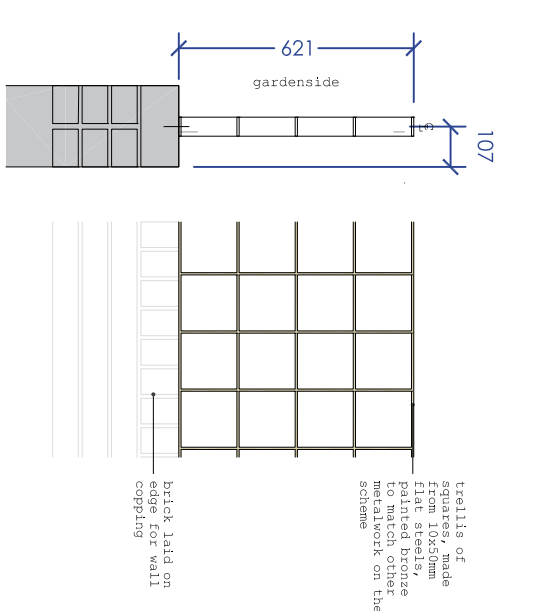
DETAIL N - boundary trellis
