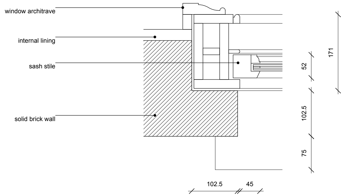
SASH WINDOW TYPICAL JAMB DETAIL
