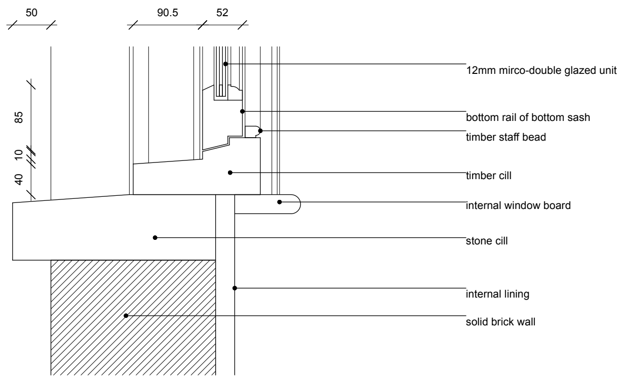
SASH WINDOW TYPICAL CILL SECTION DETAIL
