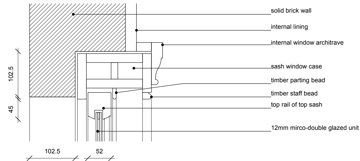
SASH WINDOW TYPICAL HEAD SECTION DETAIL
