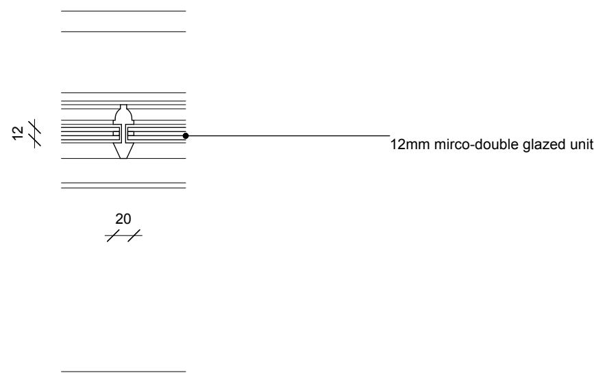
SASH WINDOW TYPICAL GLAZING BEAD DETAIL
