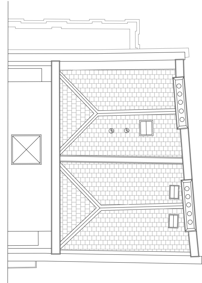
ROOF PLAN
