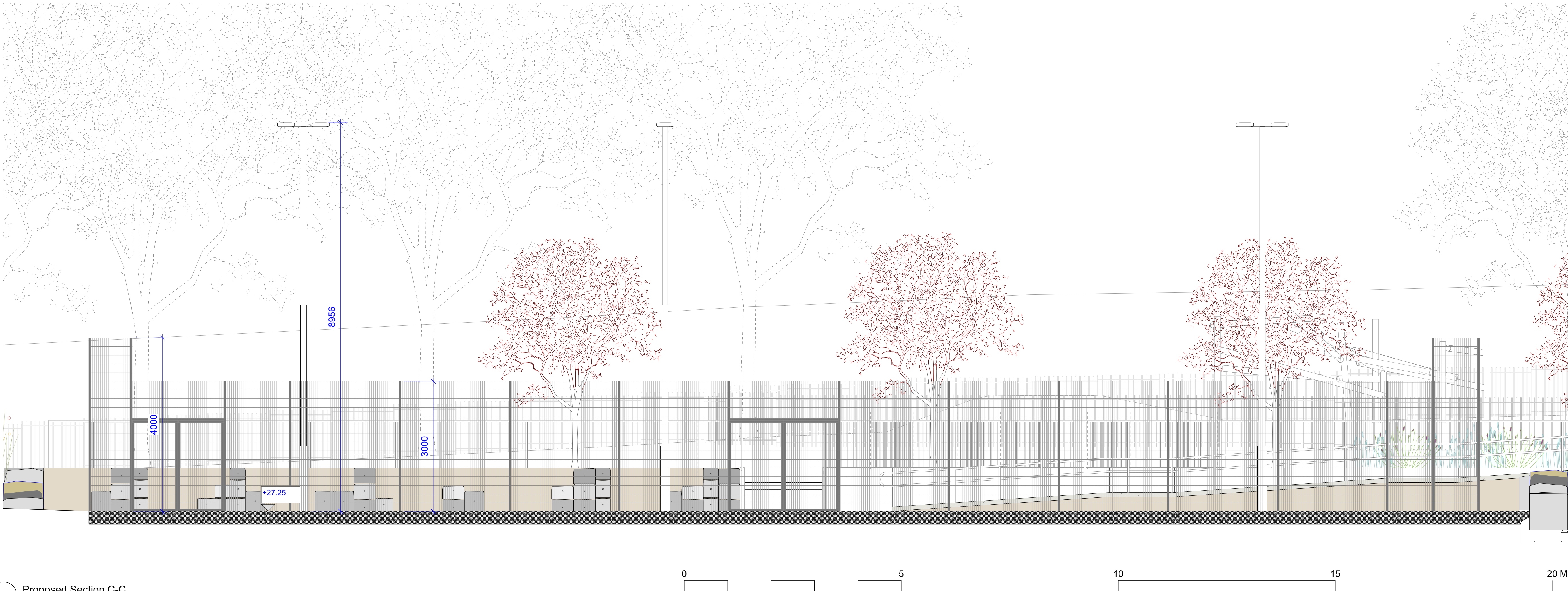
2 Proposed Section C-C Scale: 1:50
