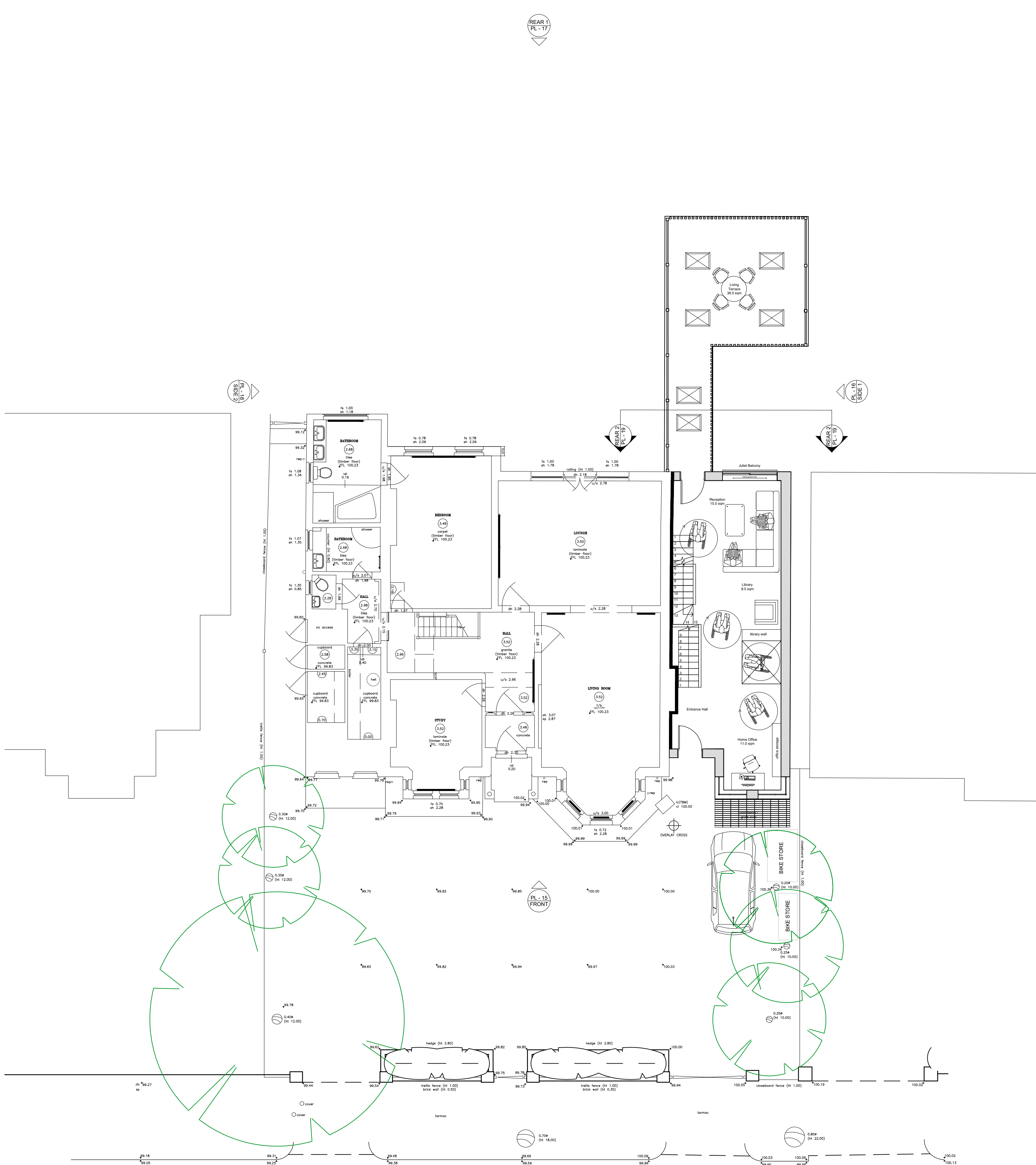
PROPOSED GROUND FLOOR
