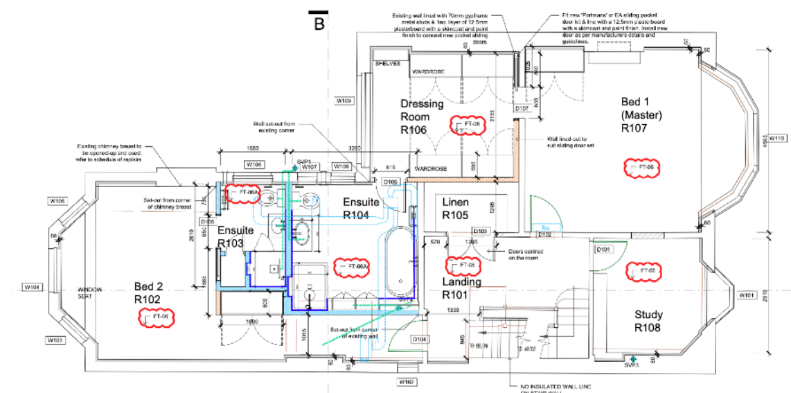
Second Floor Plan @ 1:50
