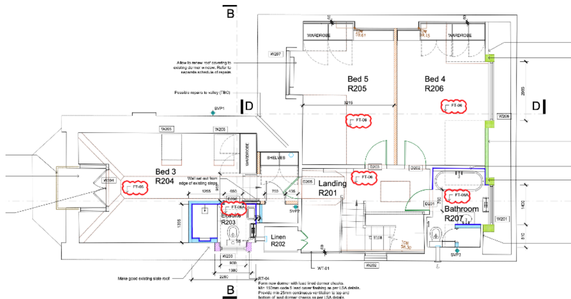
Second Floor Plan @ 1:50
