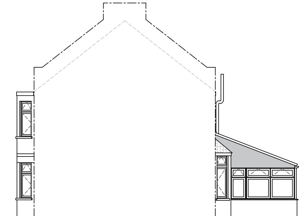
LEFT-HAND SIDE ELEVATION
