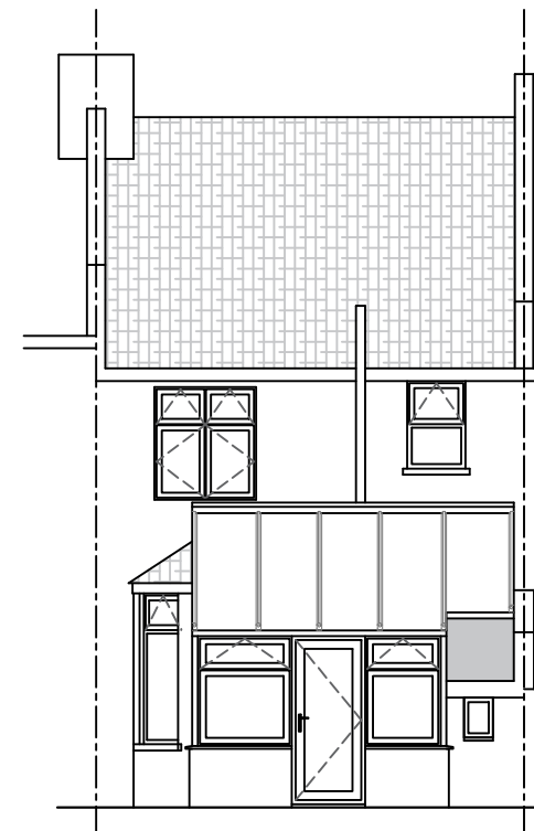
REAR ELEVATION
