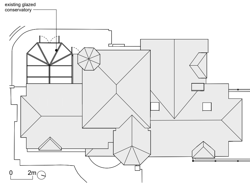
1 Roofplan Existing 1 : 200
