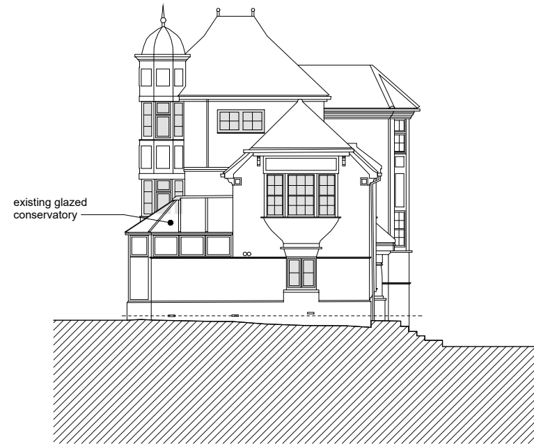
7 SOUTH elev conservatory ex 1 : 200
