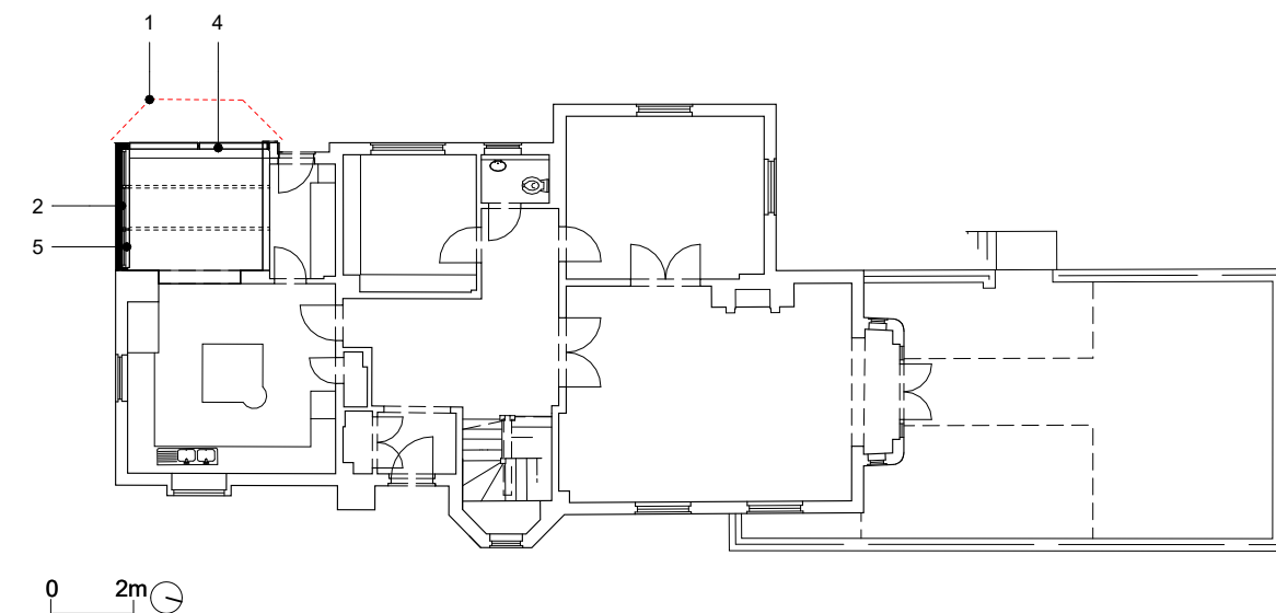
3 Level 0 proposed 1 : 200
