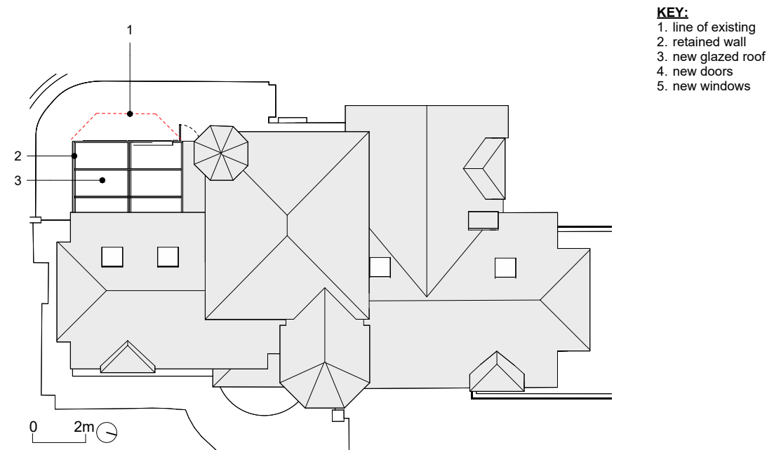
1 Roofplan Proposed 1 : 200
