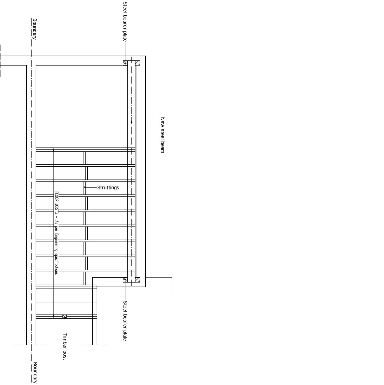
STEELWORK and JOISTS LAYOUT (Lower Landing) Scale 1:50
