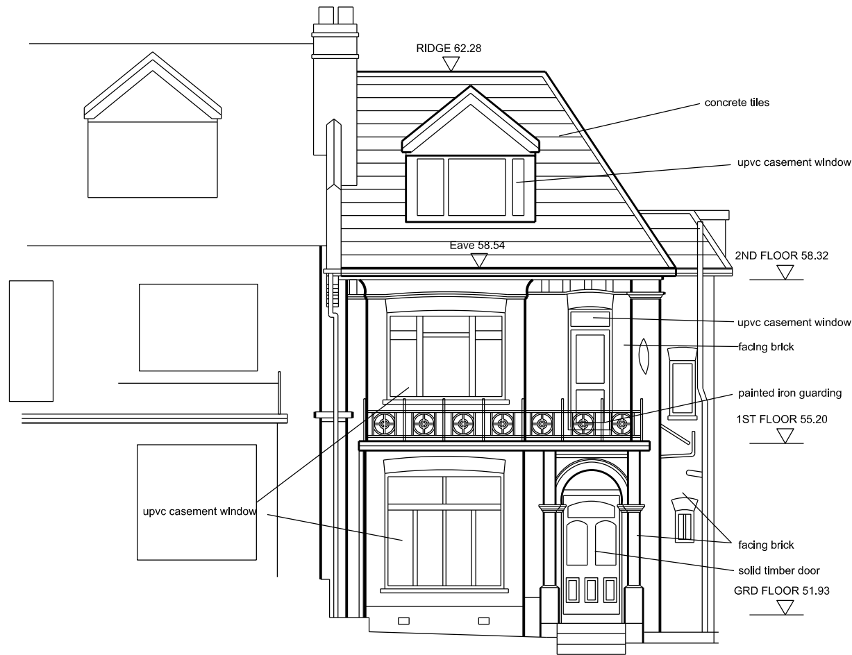
FRONT ELEVATION Existing Front Elevation DATUM LEVEL = 51.00m
