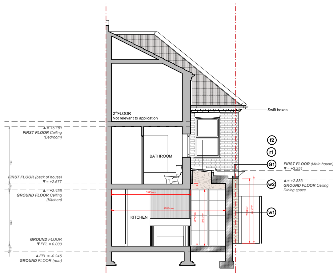
Proposed Section CC
