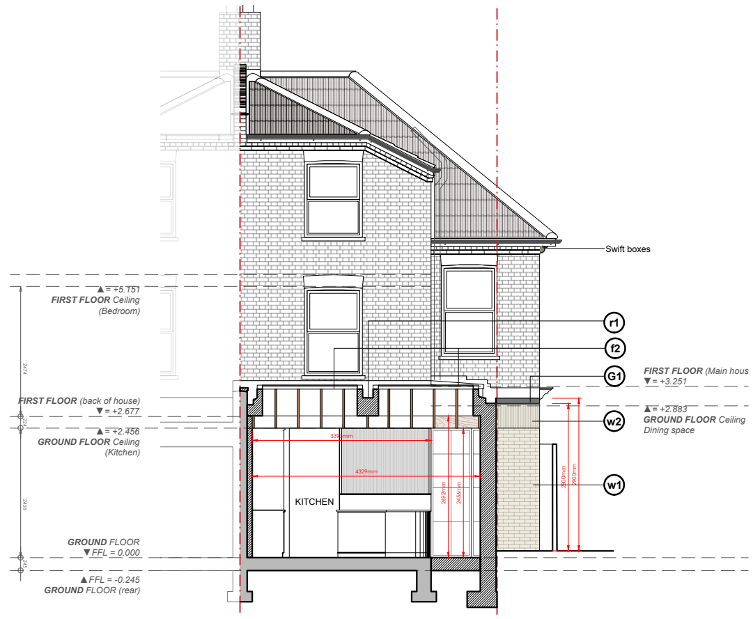
Proposed Section DD
