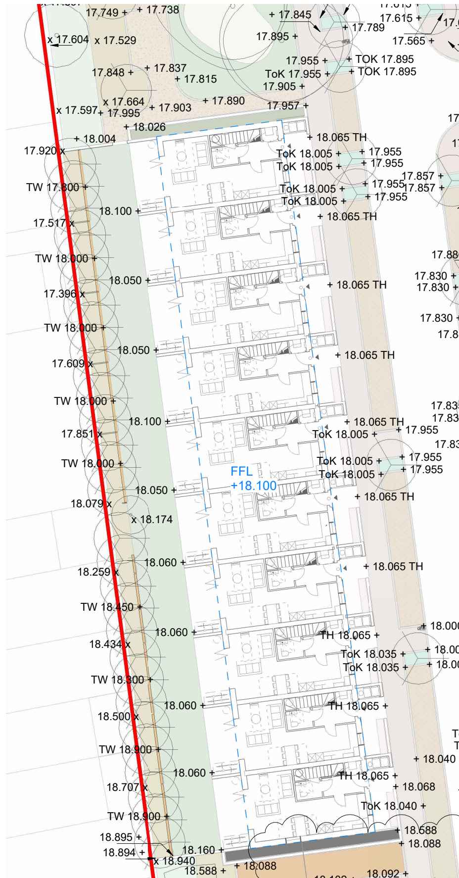
Extract of plot B1 houses taken from 'N15301-PLI-XX-ZZ-DR-L-00404'
