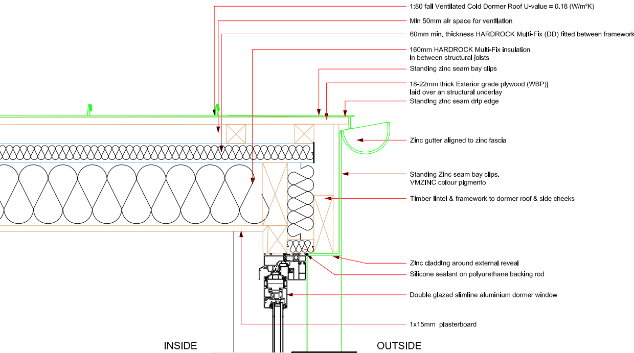
Detail 1 - Window head and reveal
