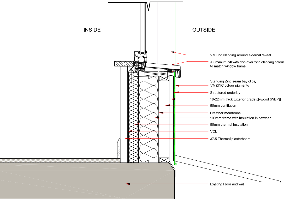
Detail 2 - Window cill base
