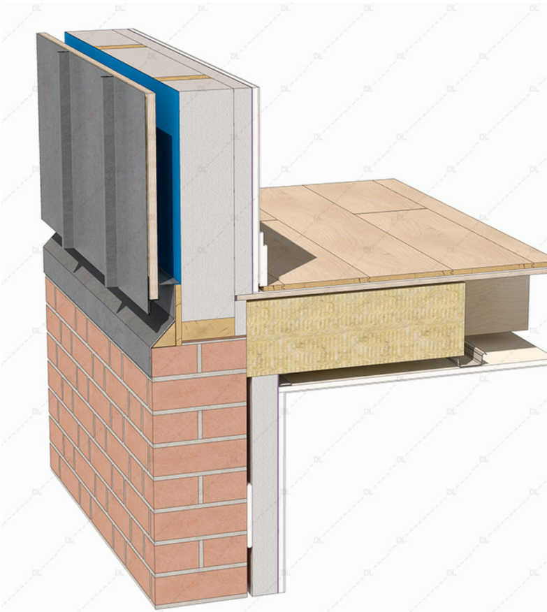
Standing Seam Zinc Base (Referential image - not to scale)
