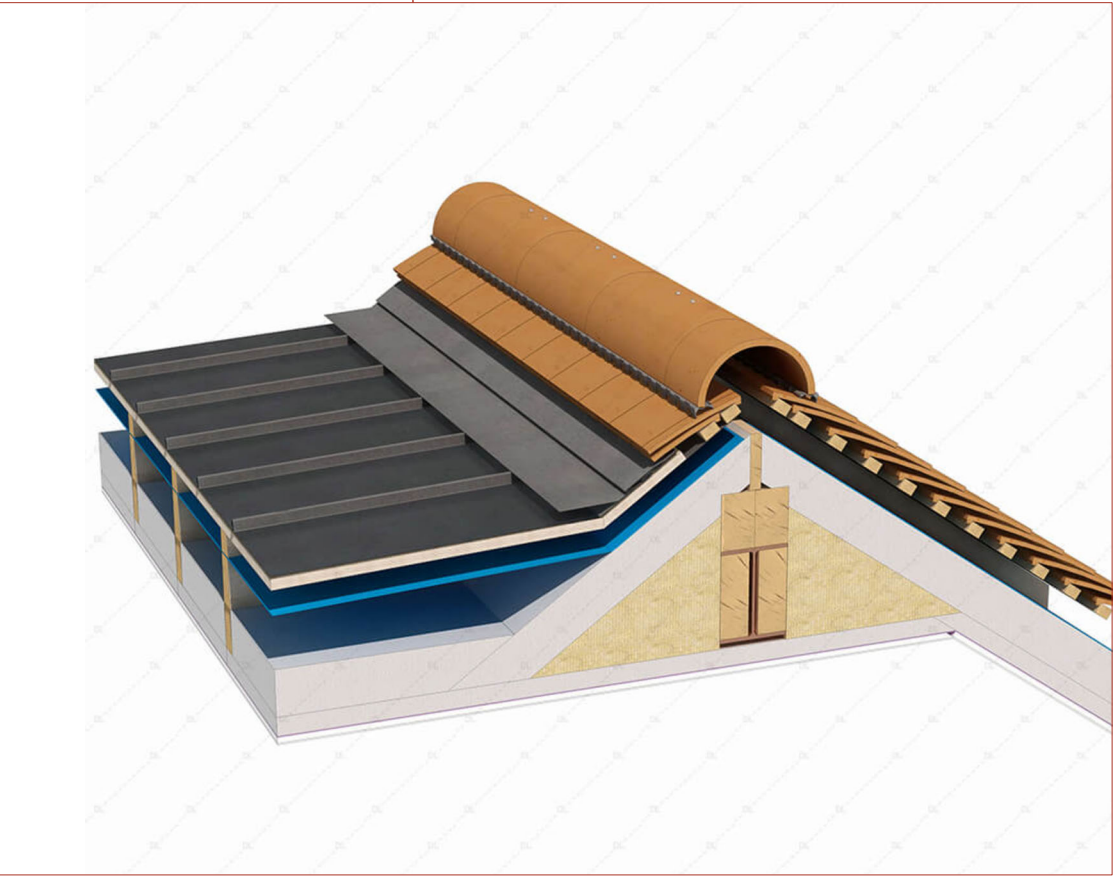
Zinc Dormer Roof Ridge Abutment with roof tiles (Referential image- not to scale)
