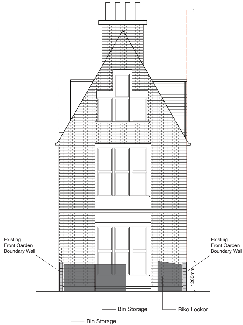
FRONT ELEVATION + Boundary Wall Section
