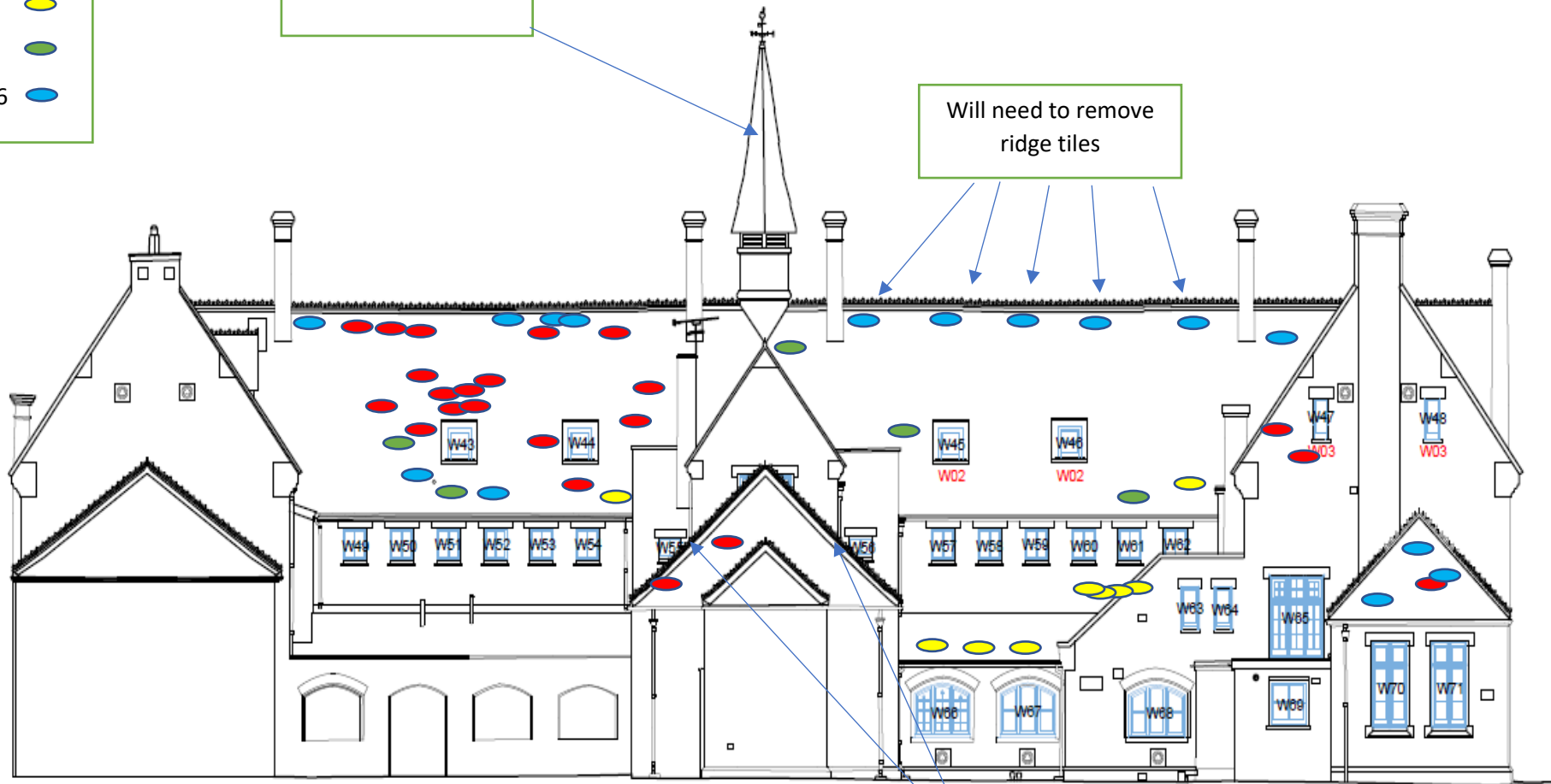
Elevation 4-4
