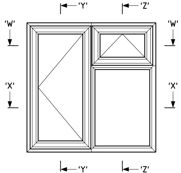
Typical Elevation (Viewed from outside) Scale 1:20
