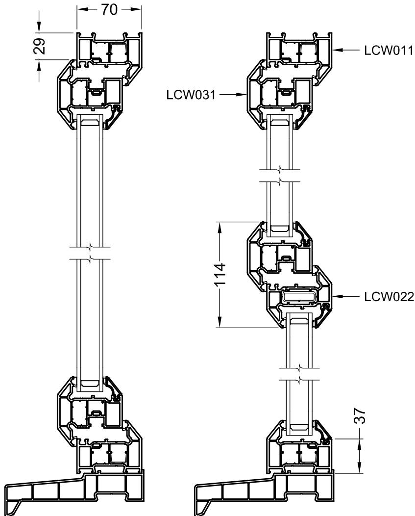
Section 'Y-Y' Scale 1:4
