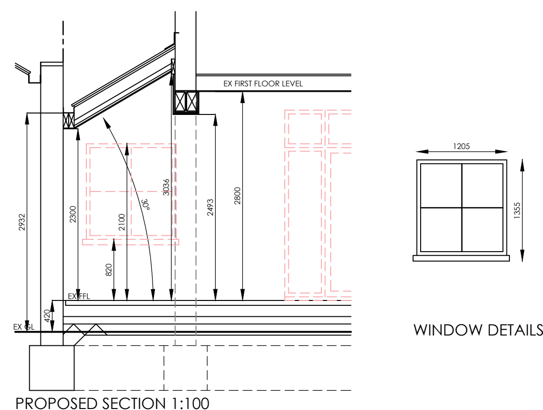
PROPOSED SECTION 1:100
