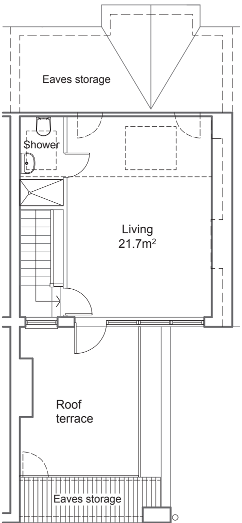
Second Floor
