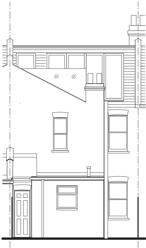
Rear Elevation
