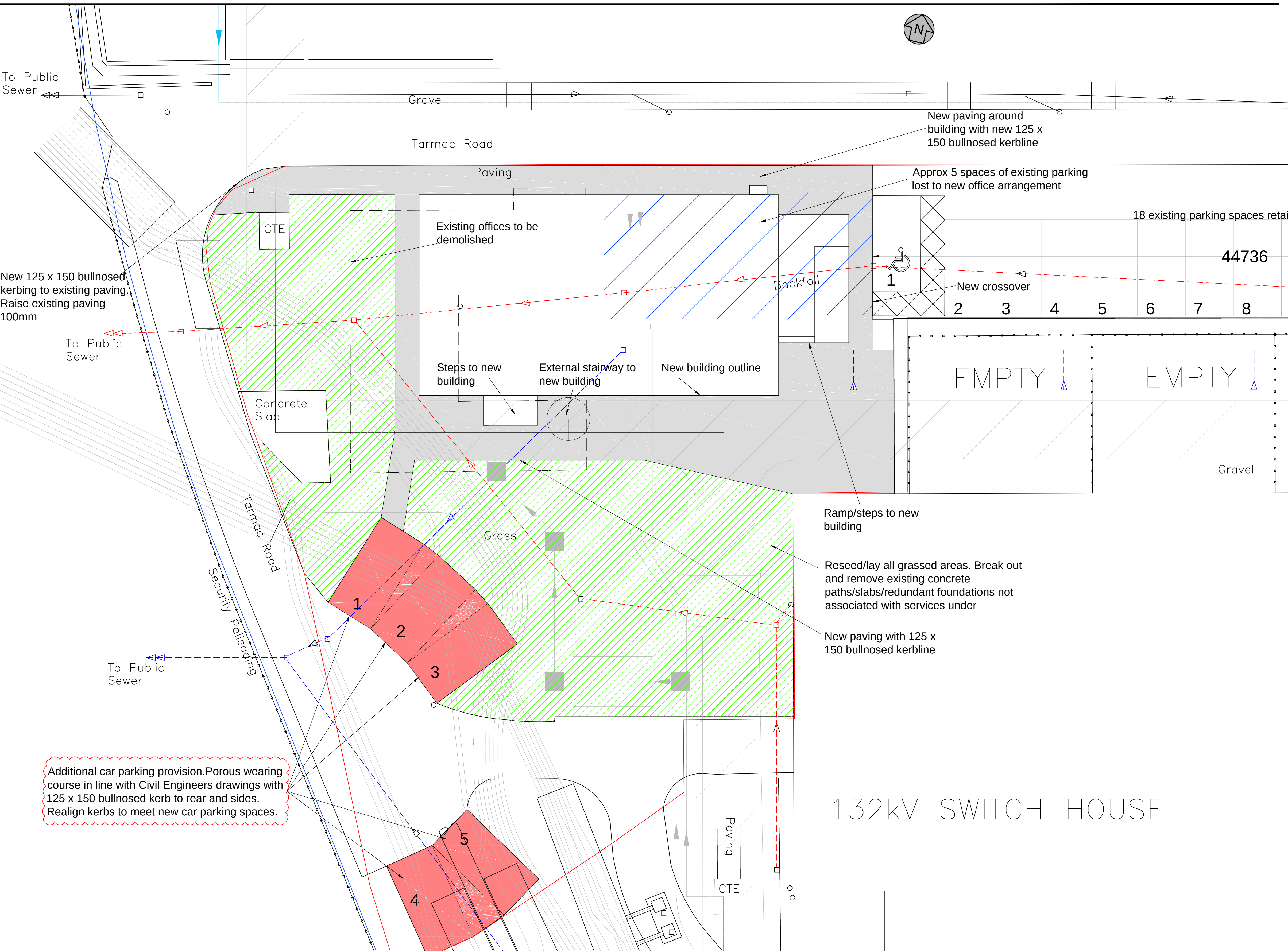
Landscaping layout (1:100@A1 1:200@A3)
