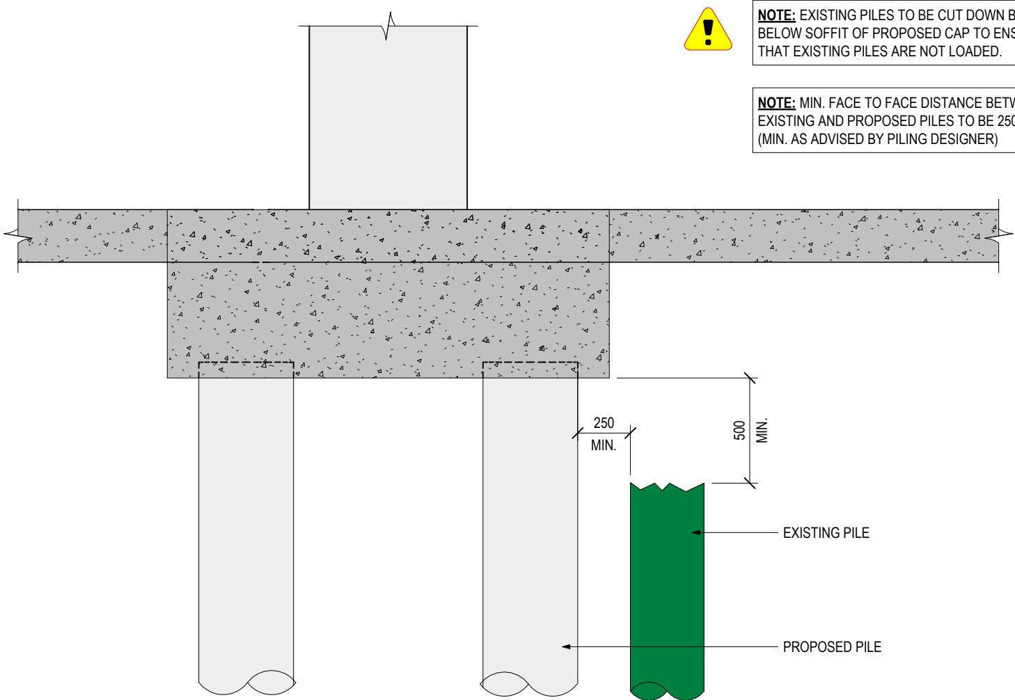
TYPICAL SECTION SHOWING THE INTERACTION BETWEEN EXISTING AND PROPOSED PILES SCALE 1:25
