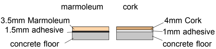
comparison of floor build up
