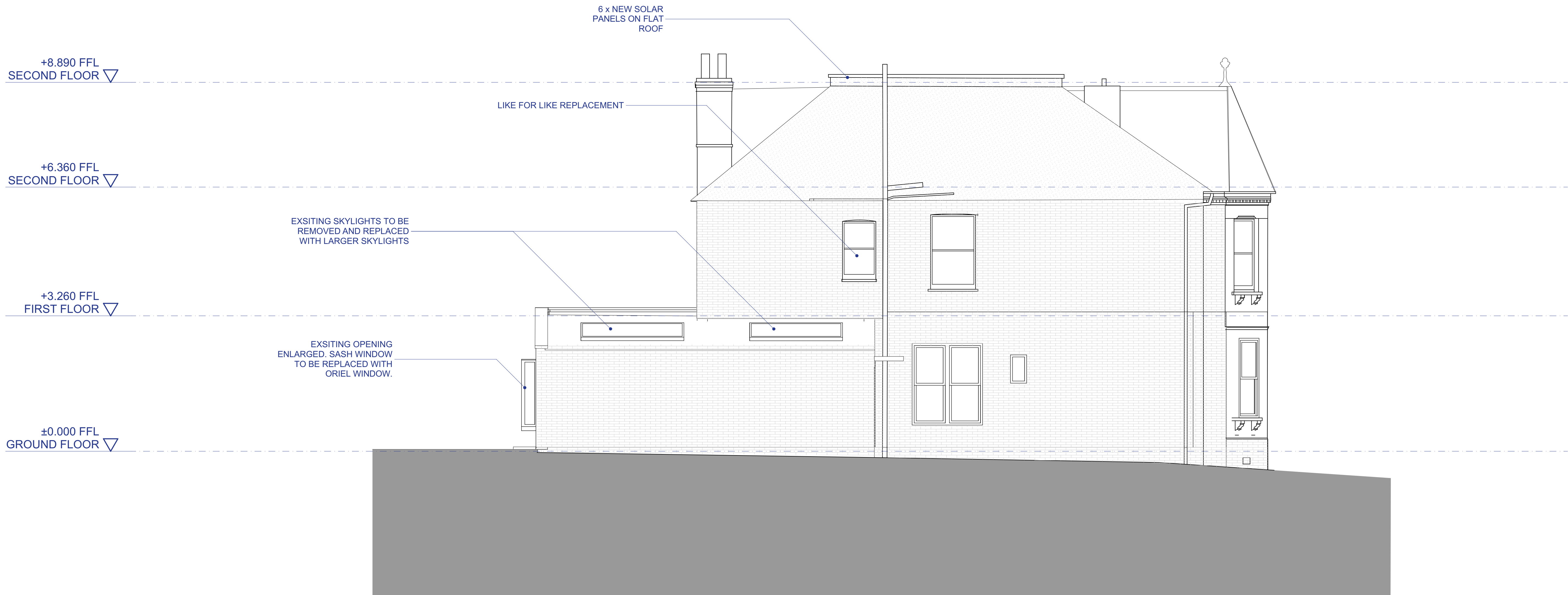
Elevation 02 - Proposed
