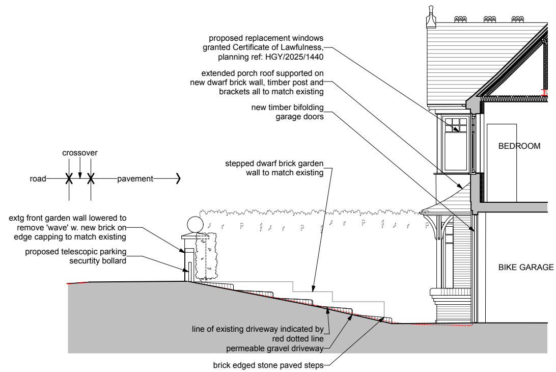
2 SECTION A.A.S PROPOSED Scale: 1:100
