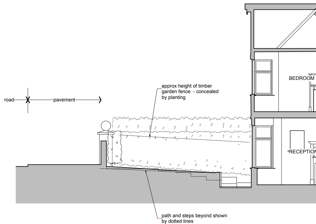
3 SECTION B.B AS EXISTING Scale: 1:100
