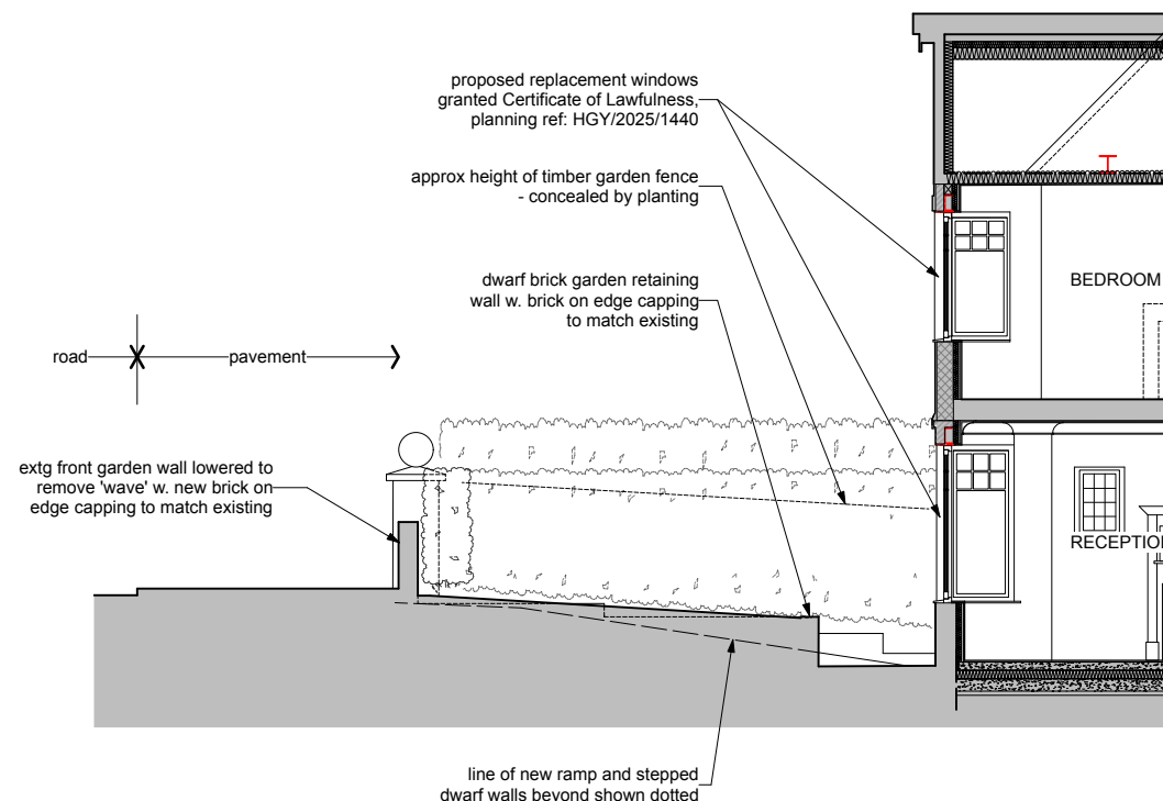
4 SECTION B.B PROPOSED Scale: 1:100
