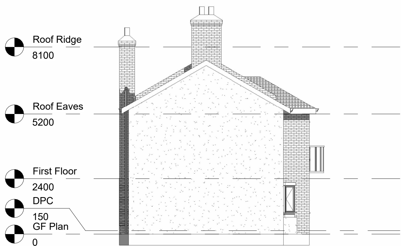
3 West Elevation Existing 1 : 100
