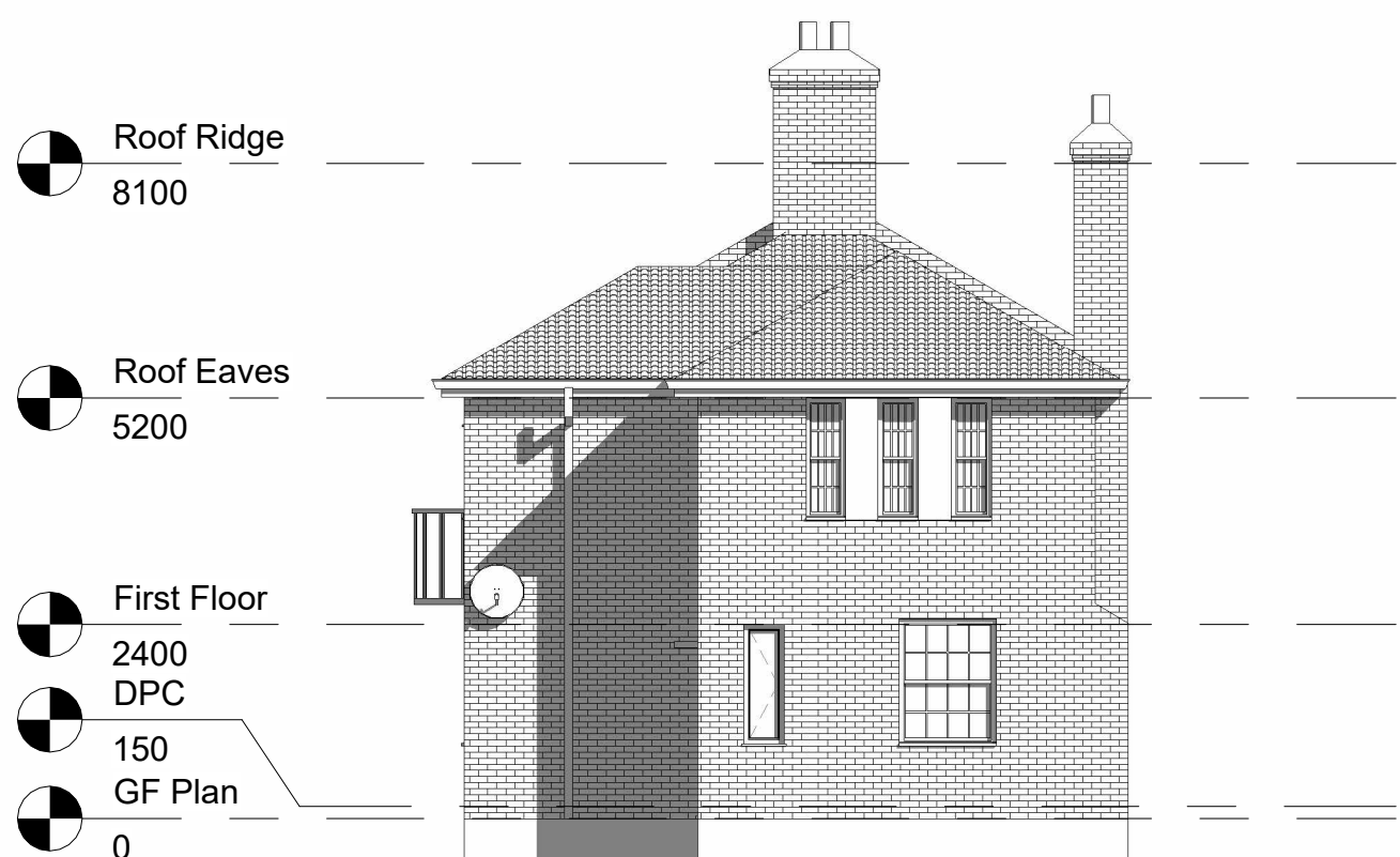
1 East Elevation Existing 1 : 100
