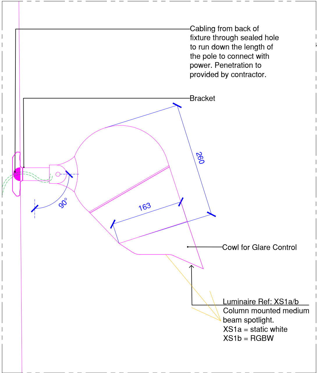
02a Column Mounted Spotlight - Mounting Detail Scale = 1:5
