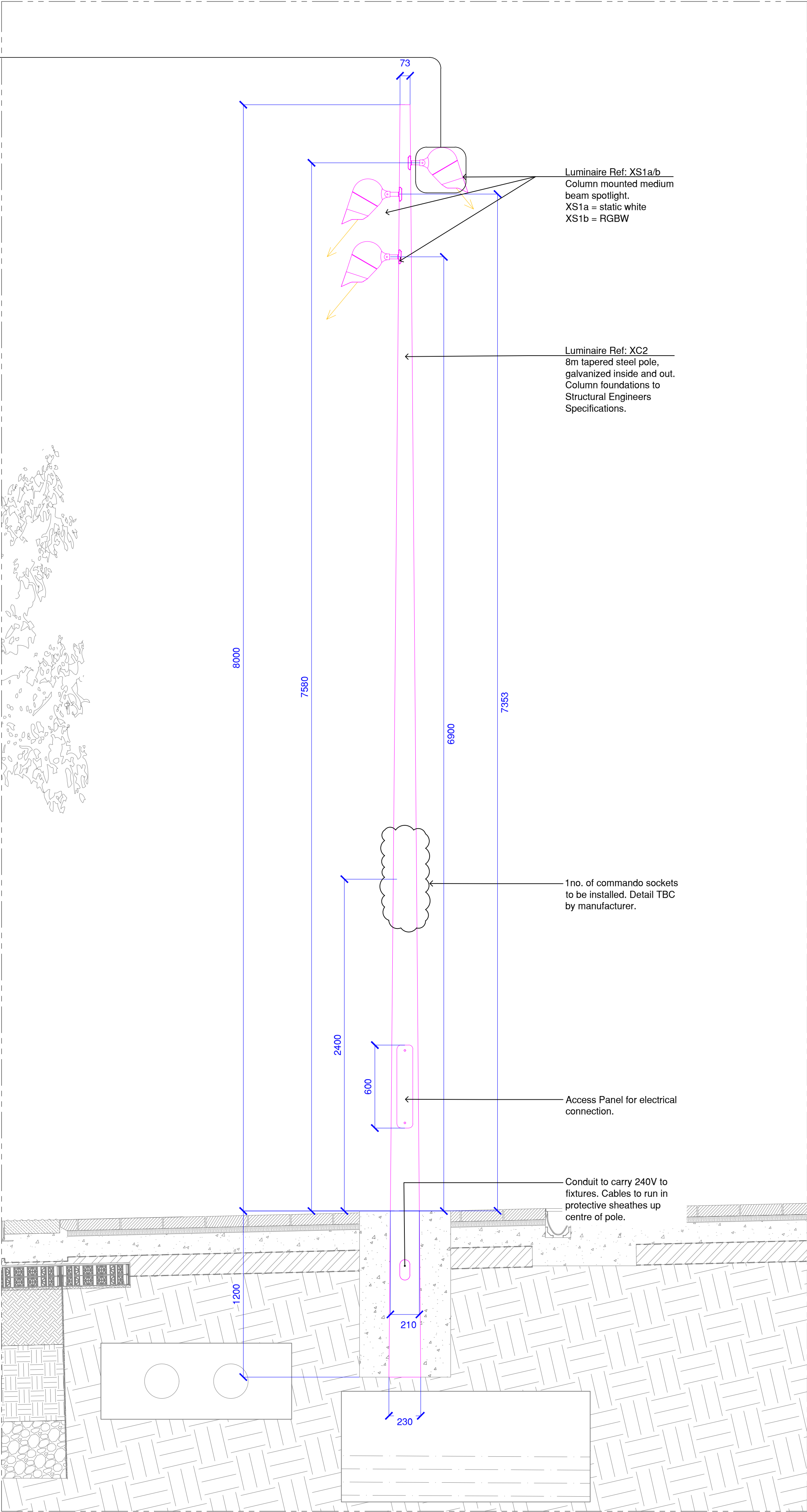
02 Column Mounted Spotlight - Lighting Detail Scale = 1:20
