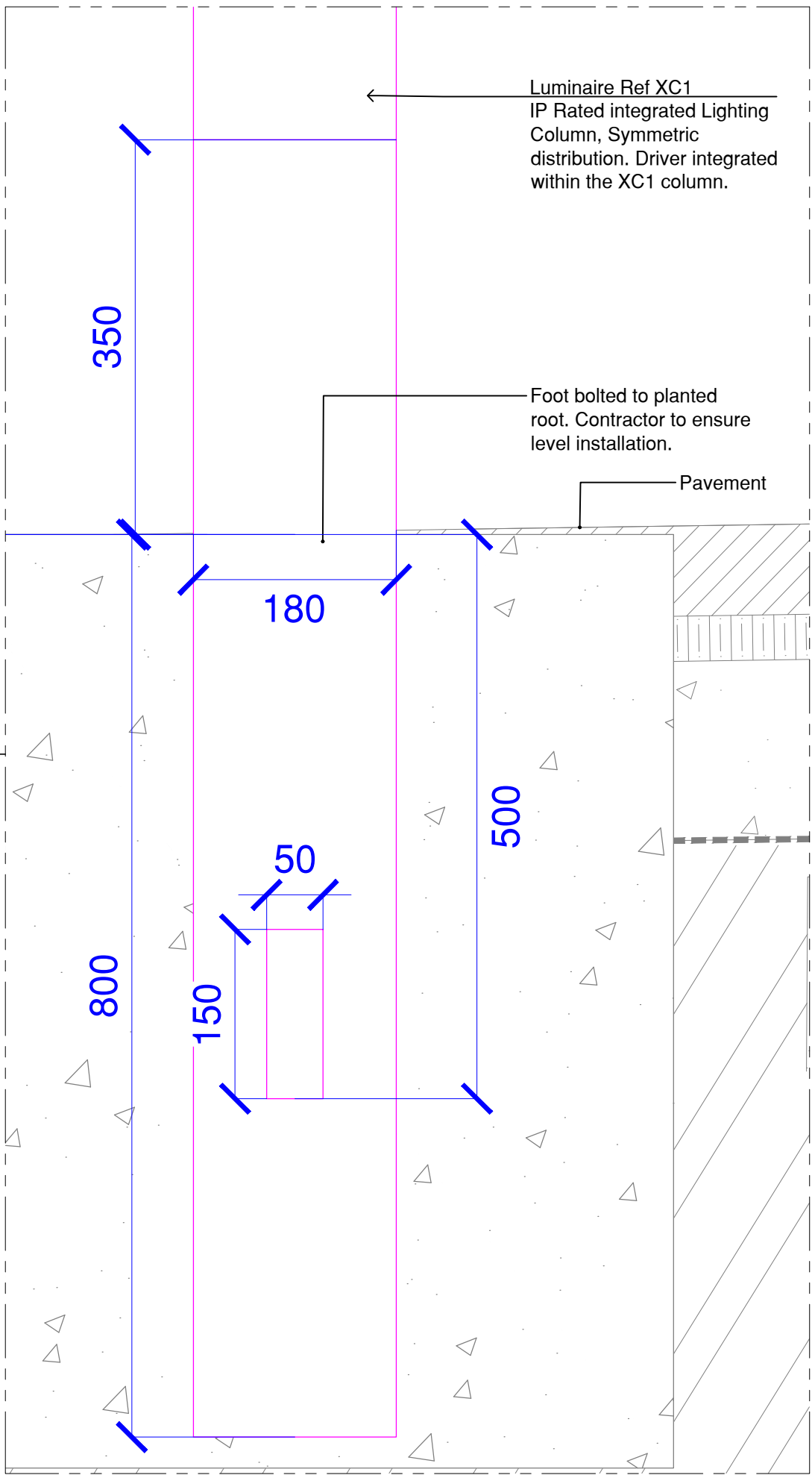
01a Light Column footing detail Scale = 1:5
