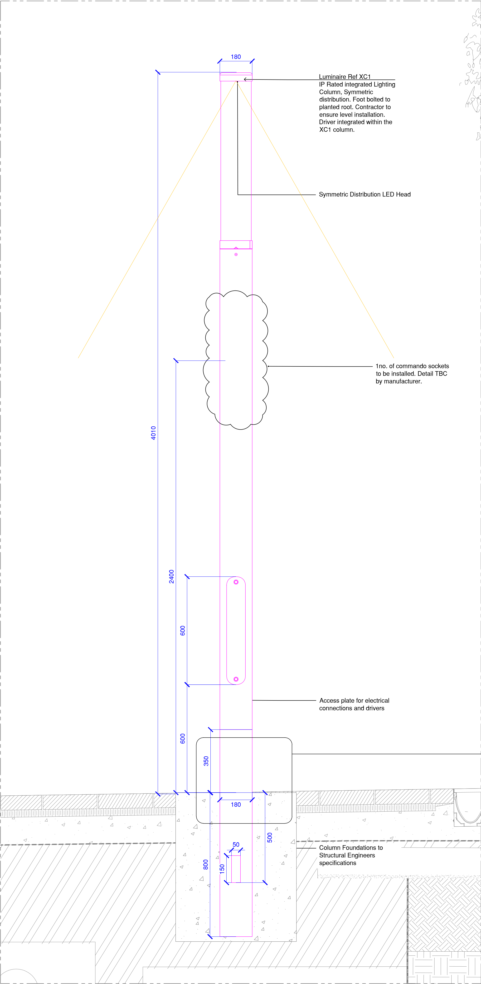
01a Column - Lighting Detail Scale = 1:10
