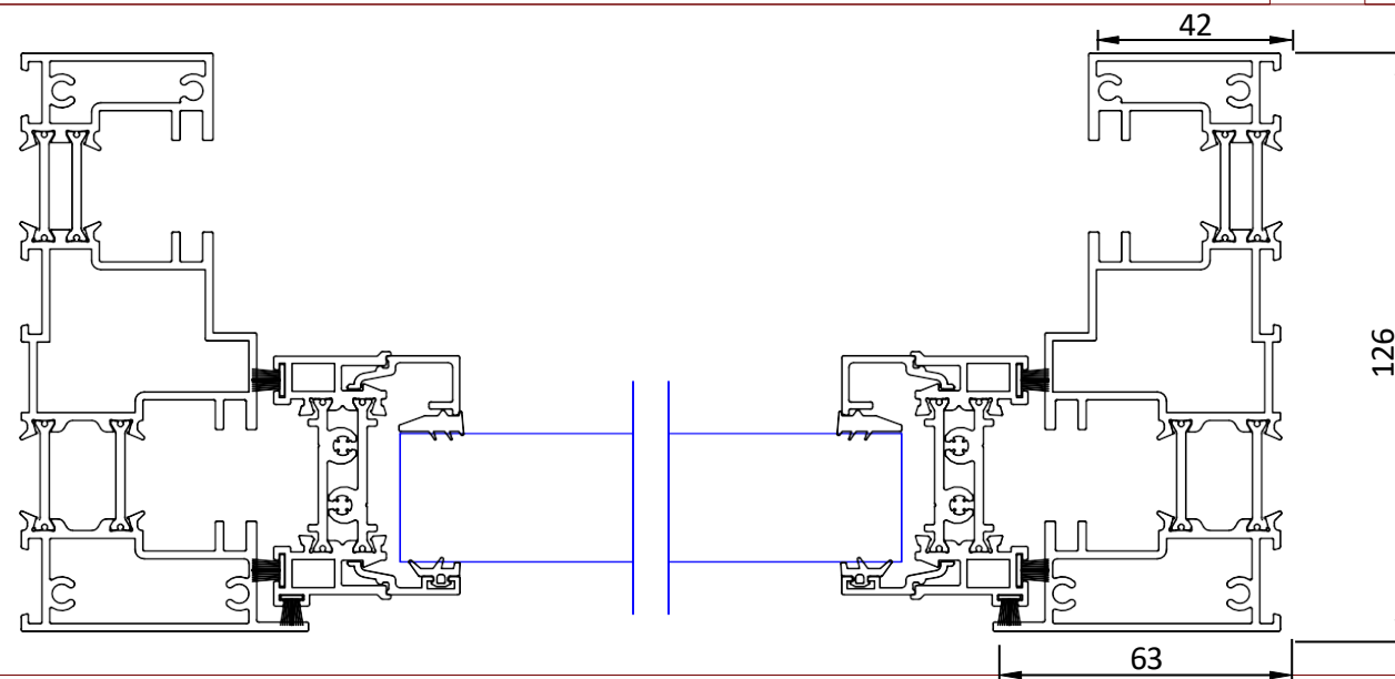
<<<<FULL WIDTH CUT THROUGH - CUT B>>>>
