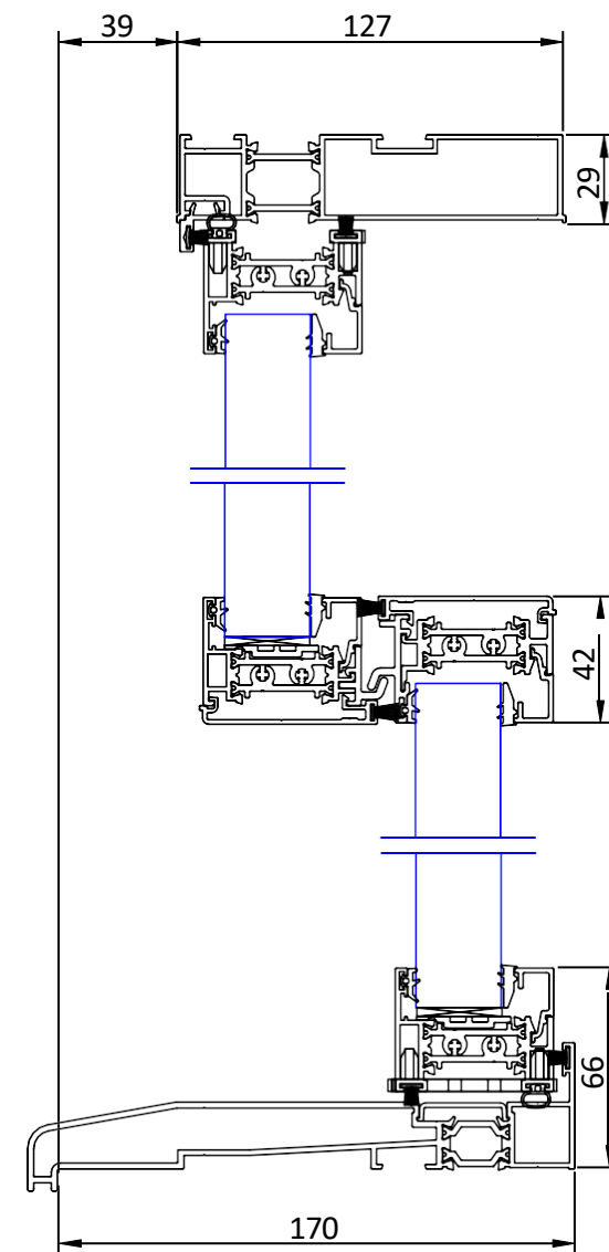
<<<<FULL HEIGHT CUT THROUGH - CUT A>>>>
