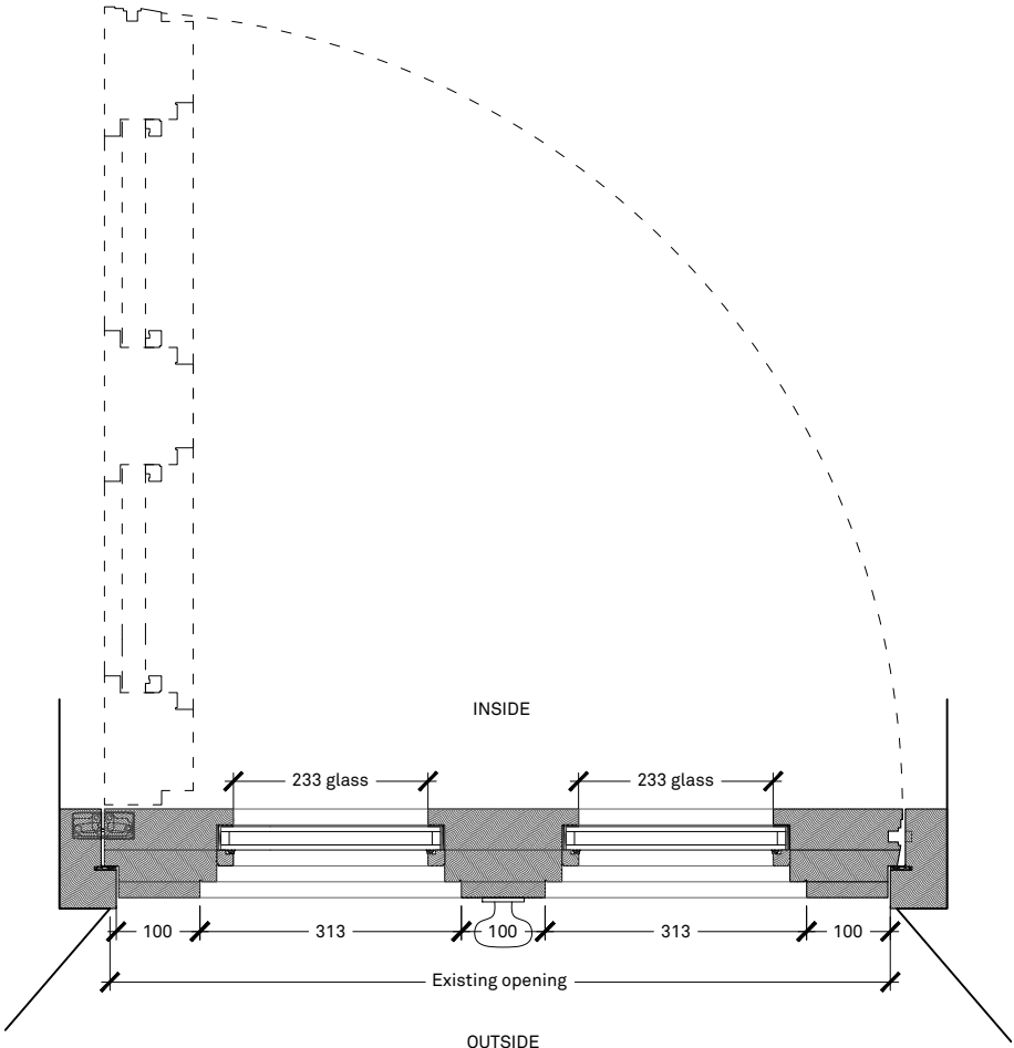
DETAILED PLAN SCALE 1:10
