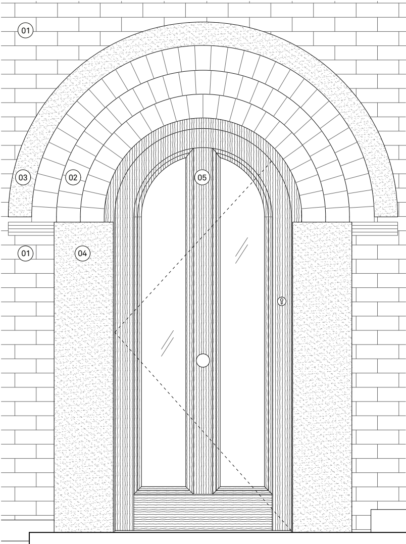
DETAILED ELEVATION SCALE 1:20
