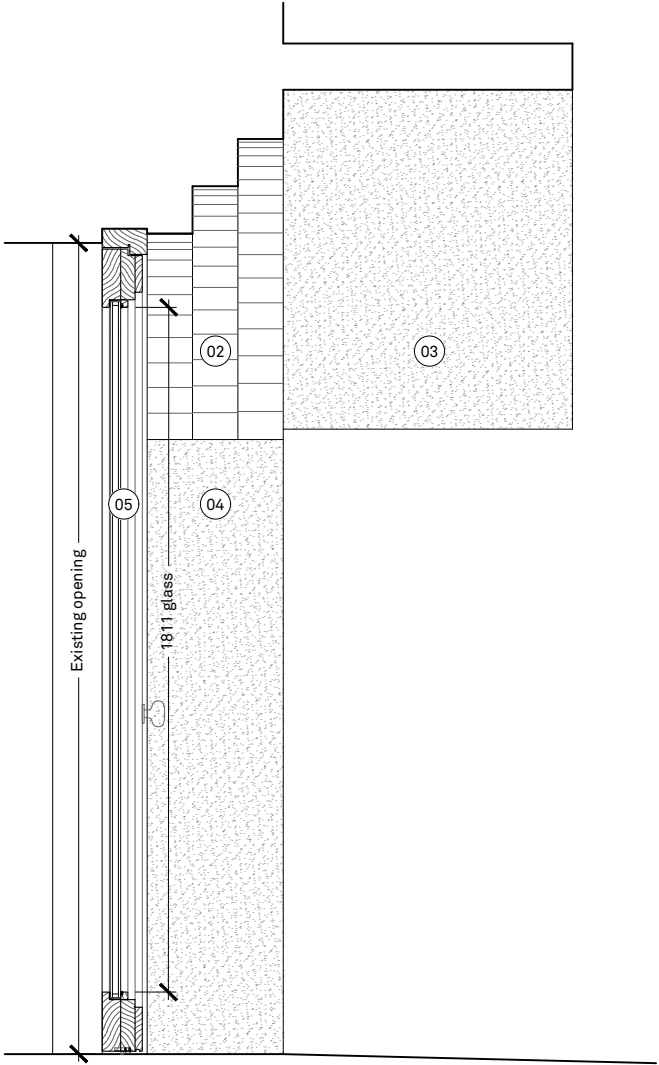
DETAILED SECTION SCALE 1:20
