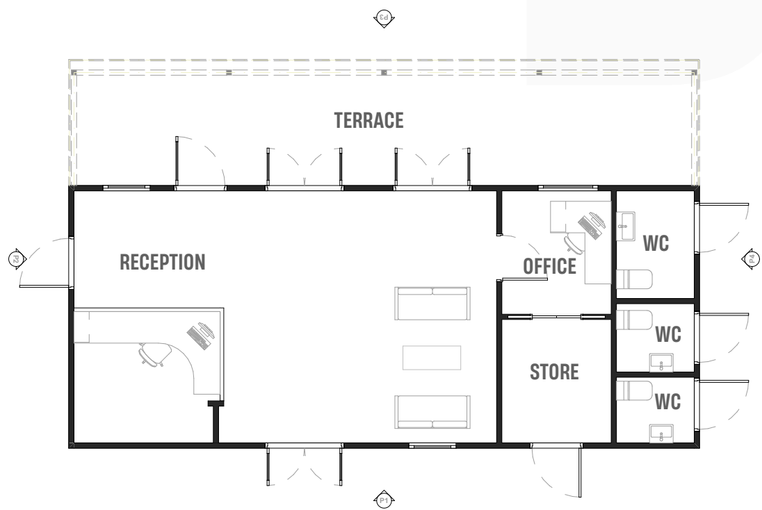
Proposed Ground Floor 1:100
