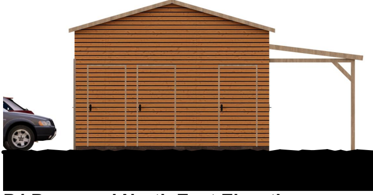
P4 Proposed North East Elevation 1:100
