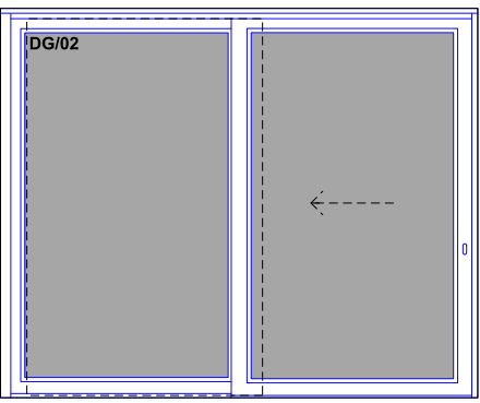
DG/02 (new) DG/02 - single sliding door
