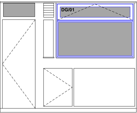
DG/01 (new) DG/01 - top-guided window / fixed window
