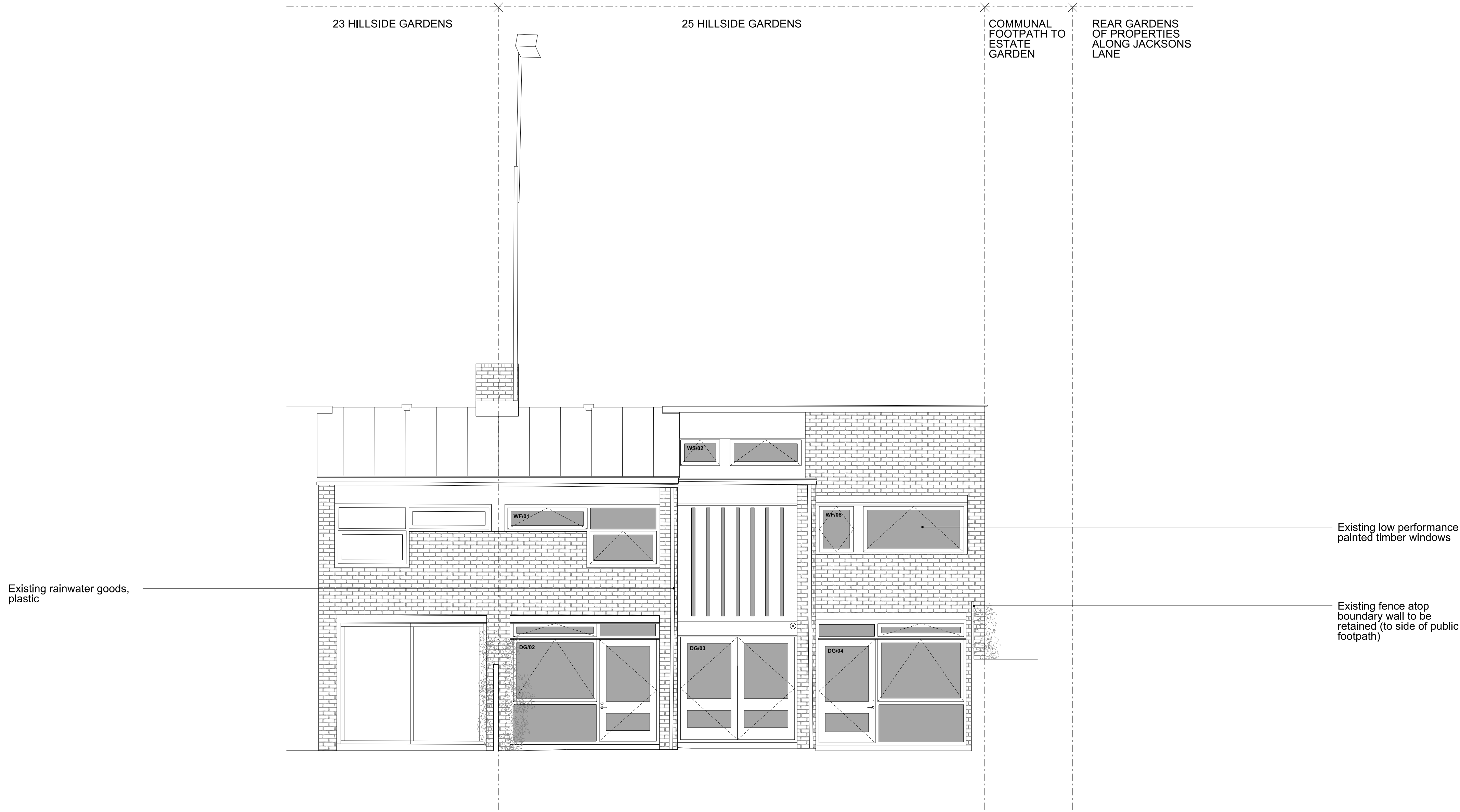
South Elevation (Rear)
