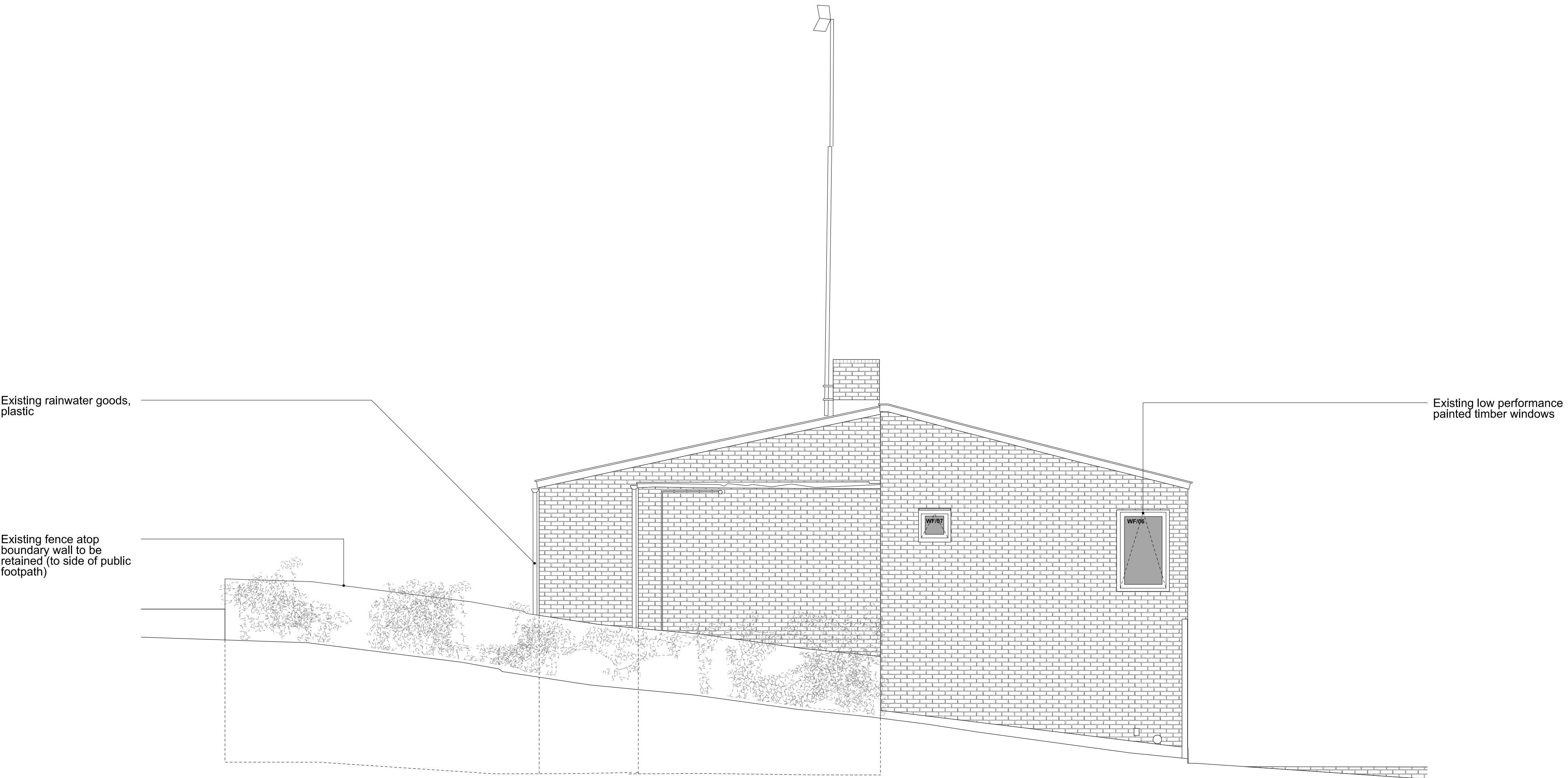
East Elevation
