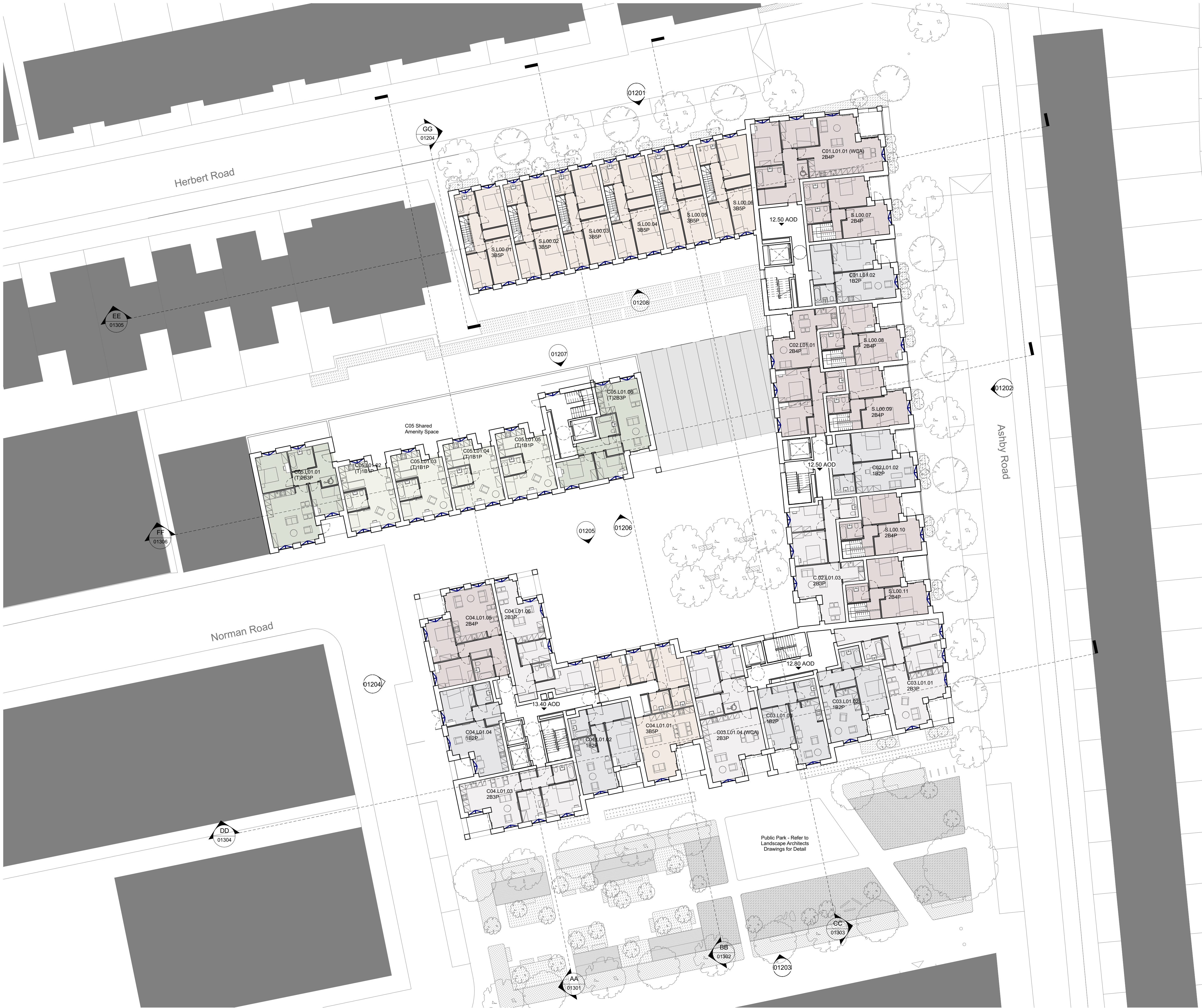
Full GA First Floor (A244-DMA-ZZ-ZZZ-DR-A-01103) Scale 1:200@A1
