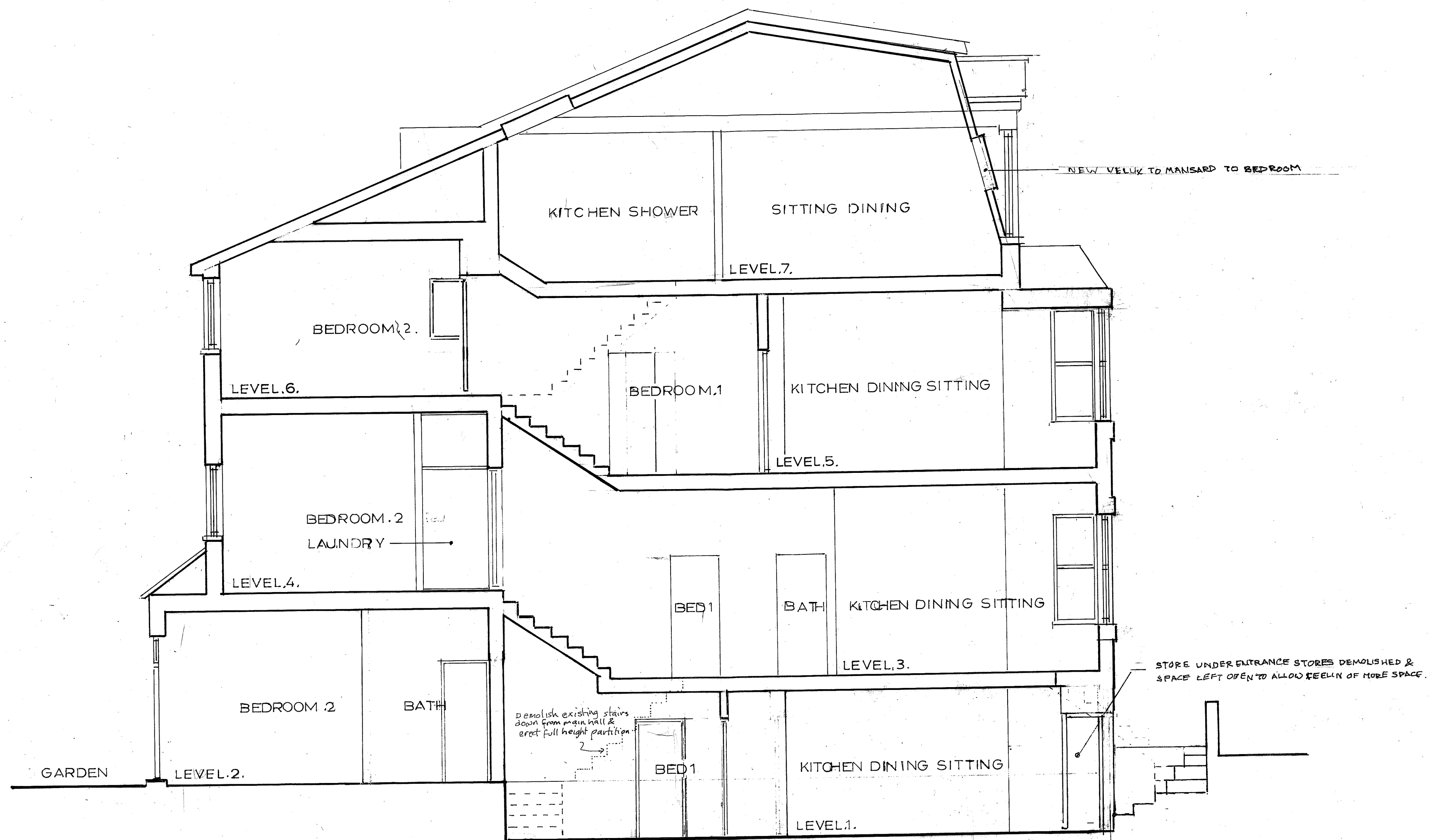
PROPOSED SECTION 'B-B' SCALE 1:50 @ A2
