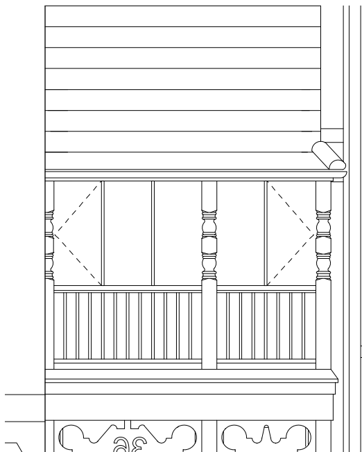
Proposed Detail 1:50
