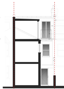
PROPOSED SECTION A-A
