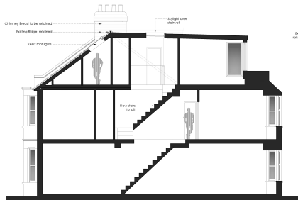
PROPOSED SECTION B-B
