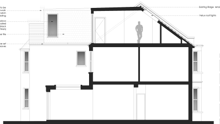
PROPOSED SECTION C-C
