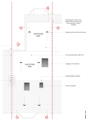
PROPOSED ROOF PLAN Scale 1:50
