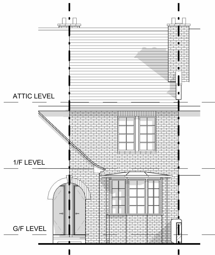
1 EXISTING SOUTH ELEVATION
