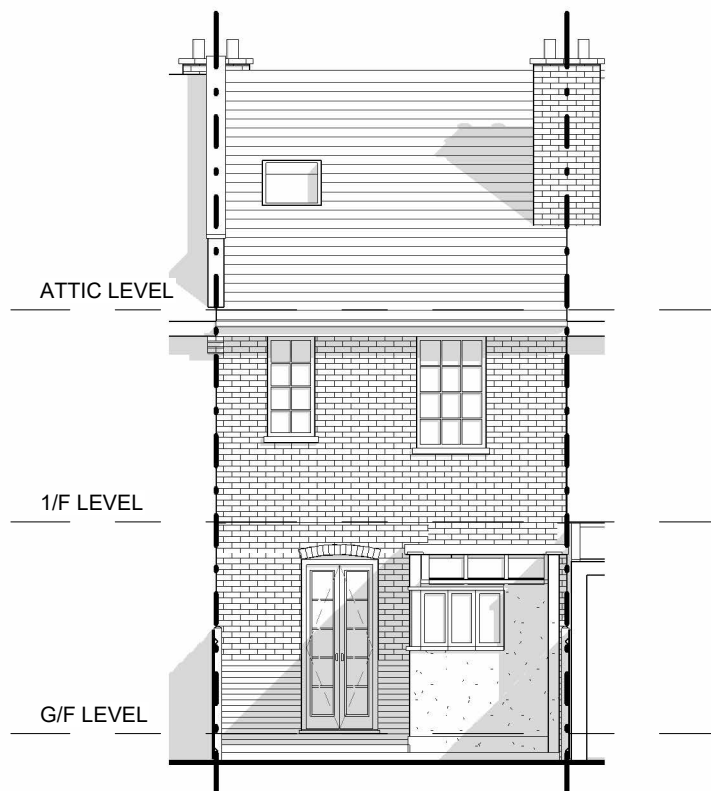
3 EXISTING NORTH ELEVATION
