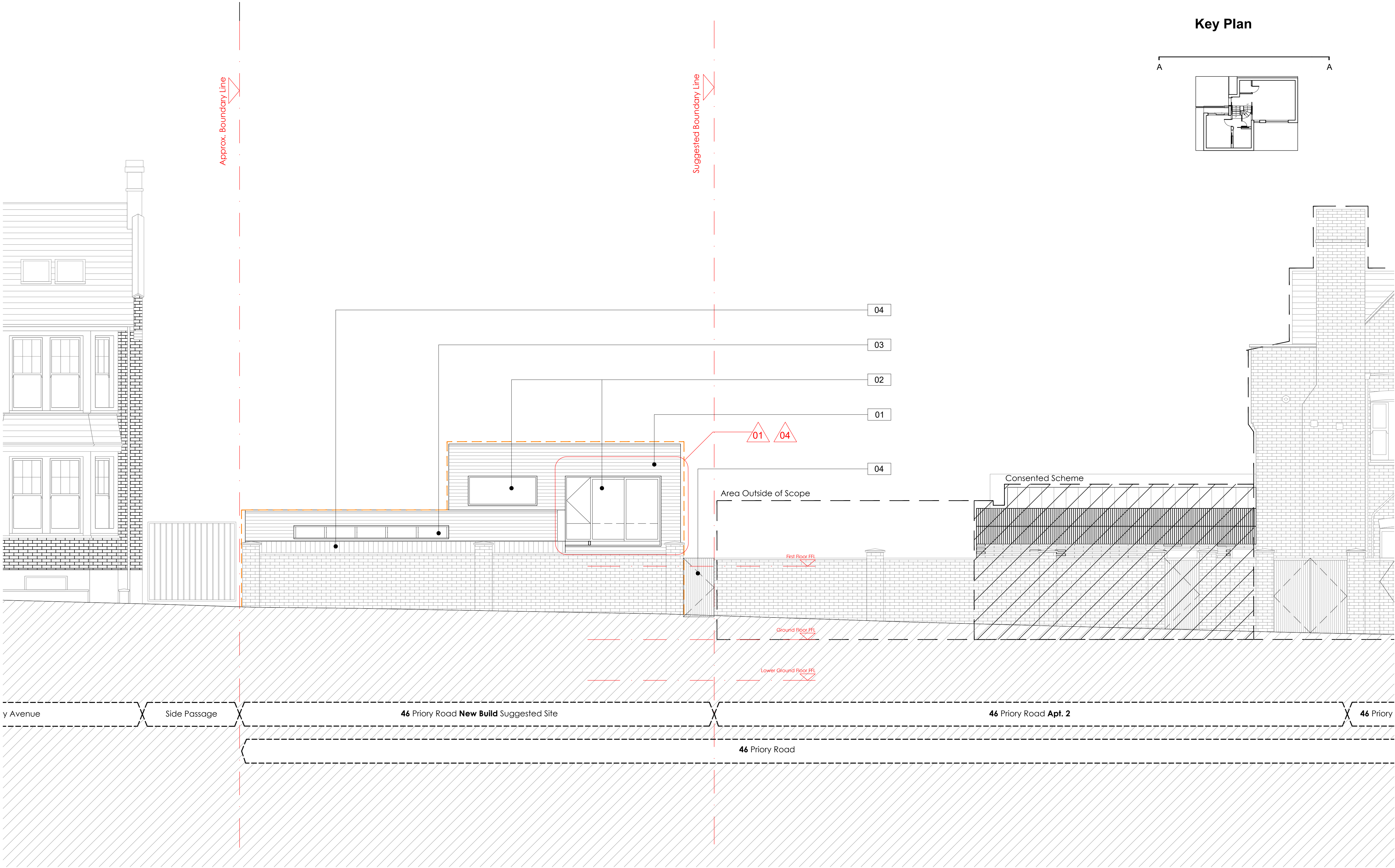
Proposed Elevation A-A
