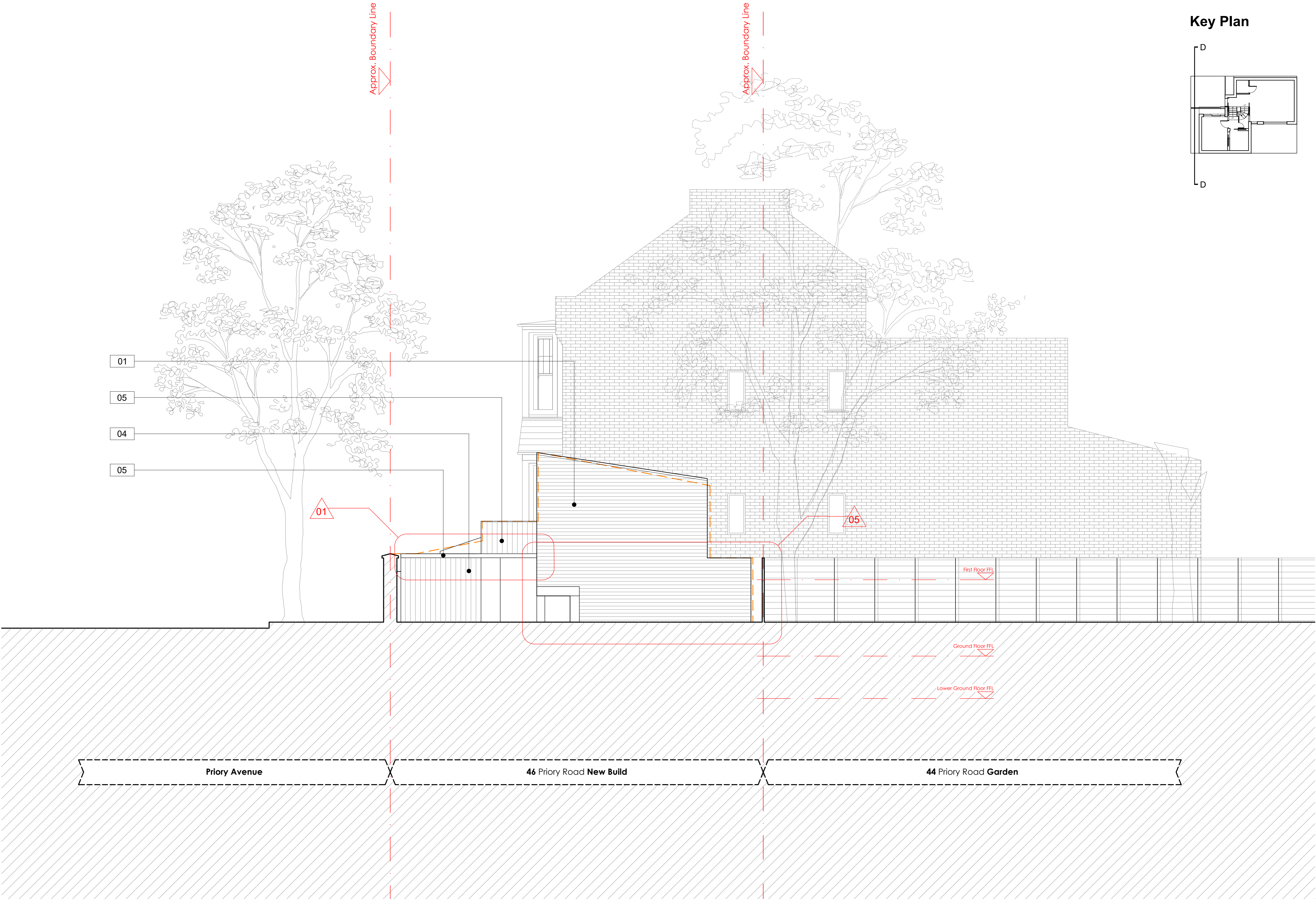
Proposed Elevation D-D
