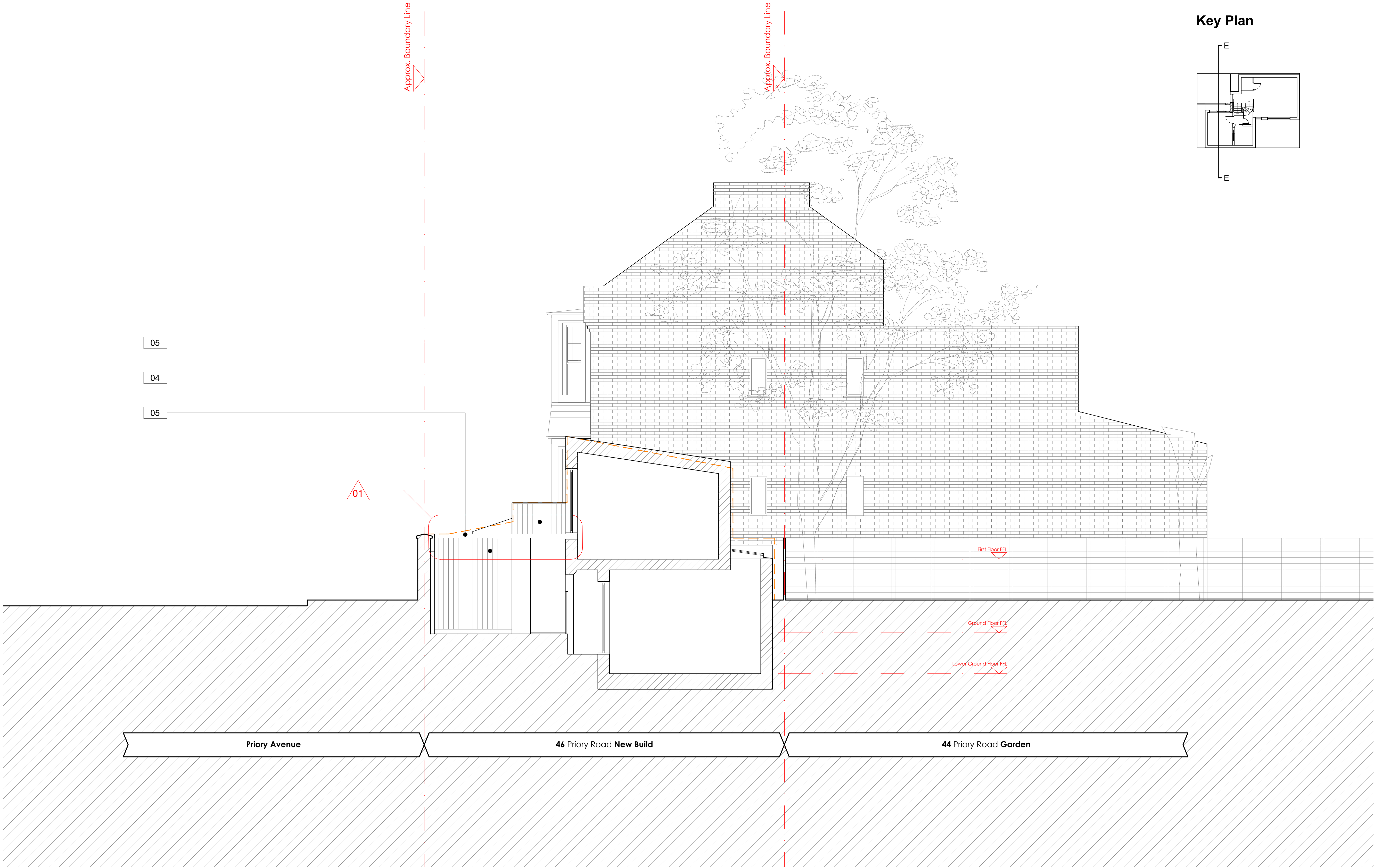
Proposed Section E-E
