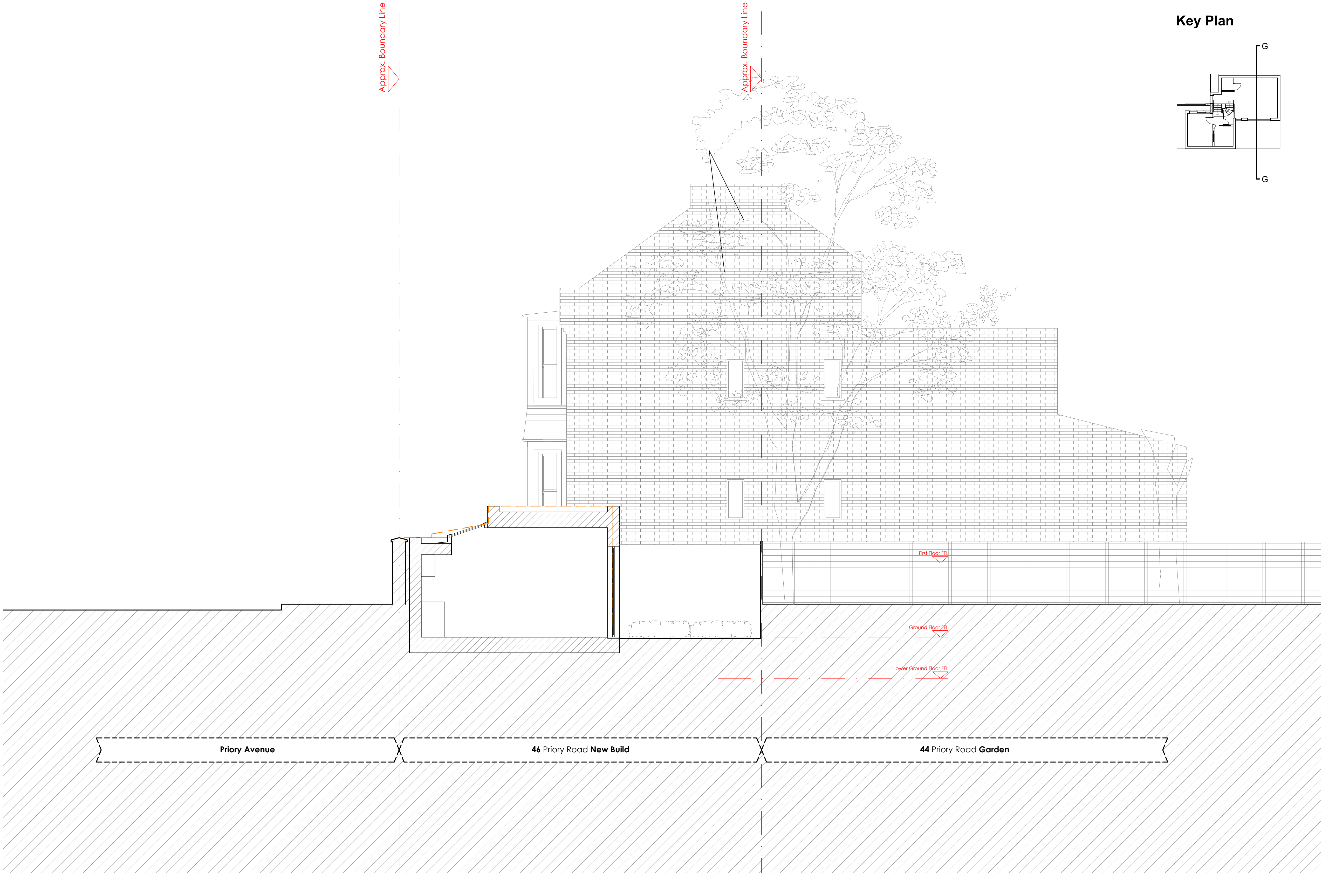
Proposed Section G-G
