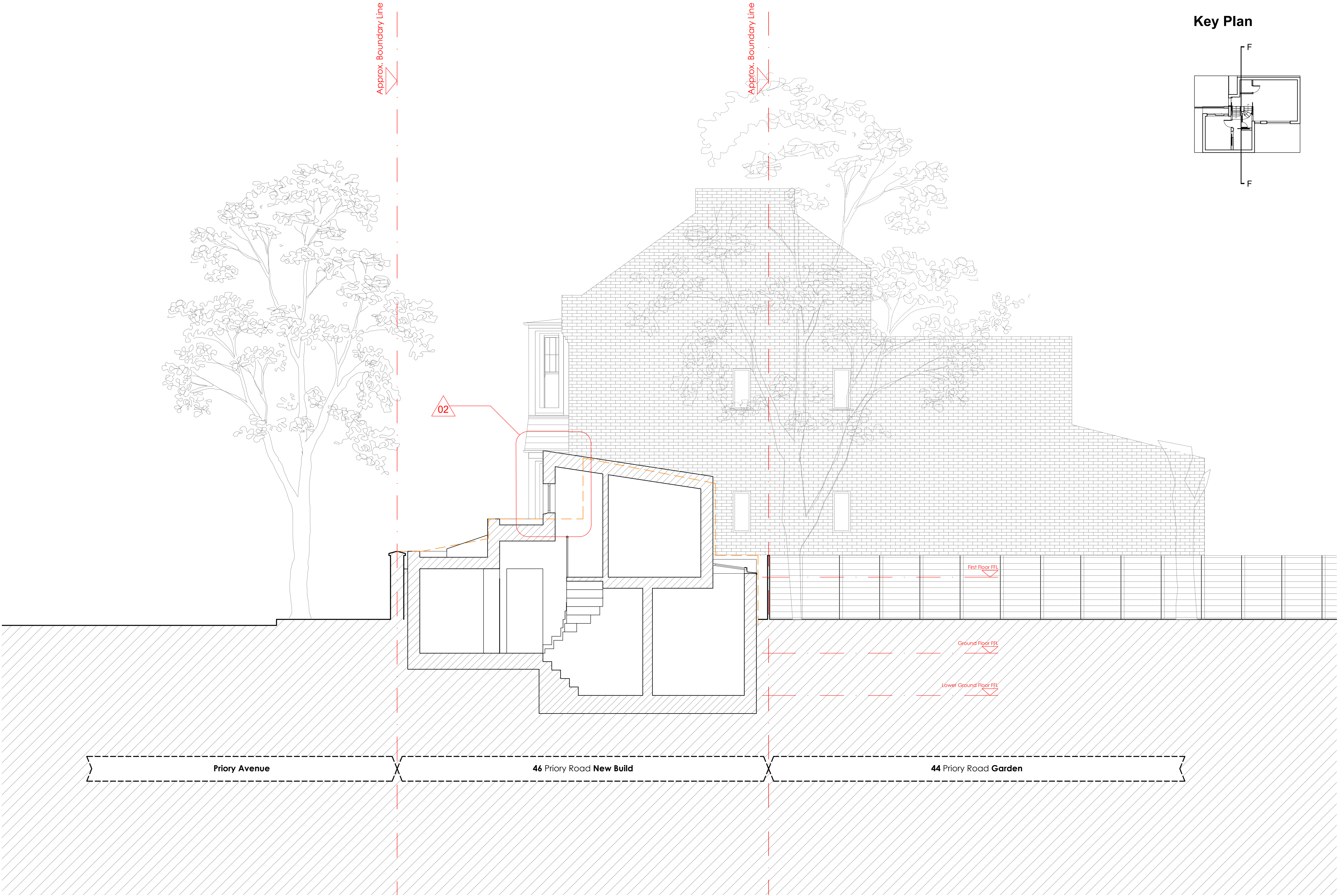
Proposed Section F-F
