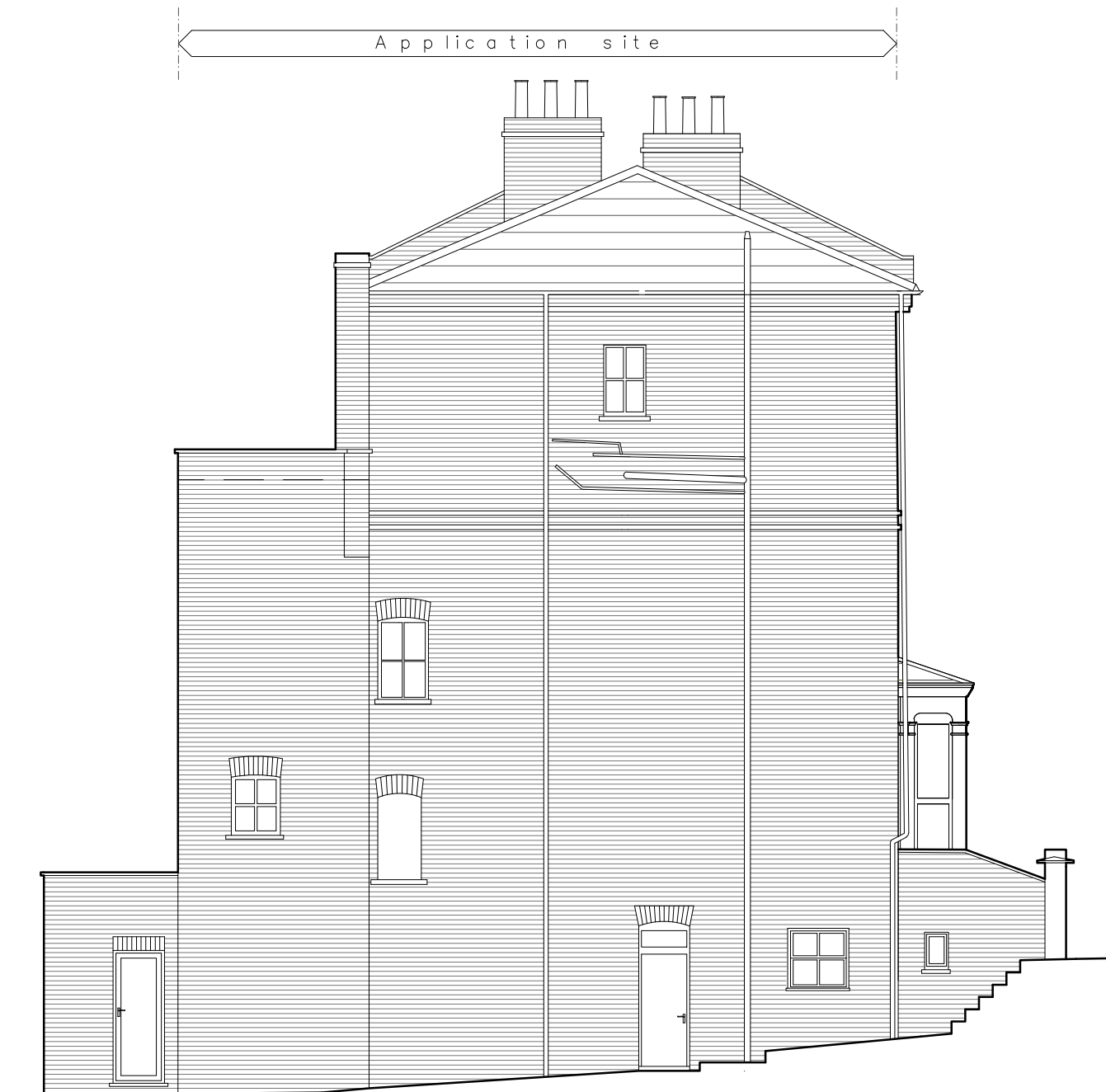
Existing Side Elevation 1:100 @ A3
