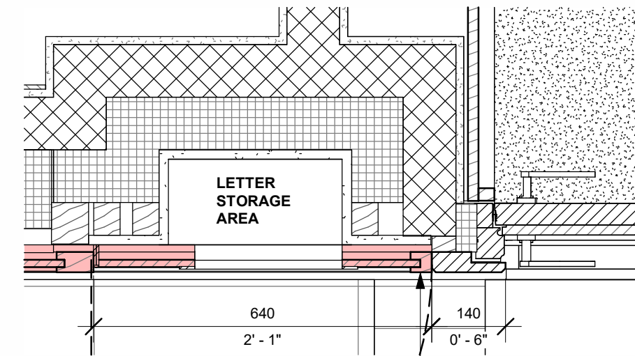
W13 & W17 JAMB DETAILS (LOWER PLAN A)
