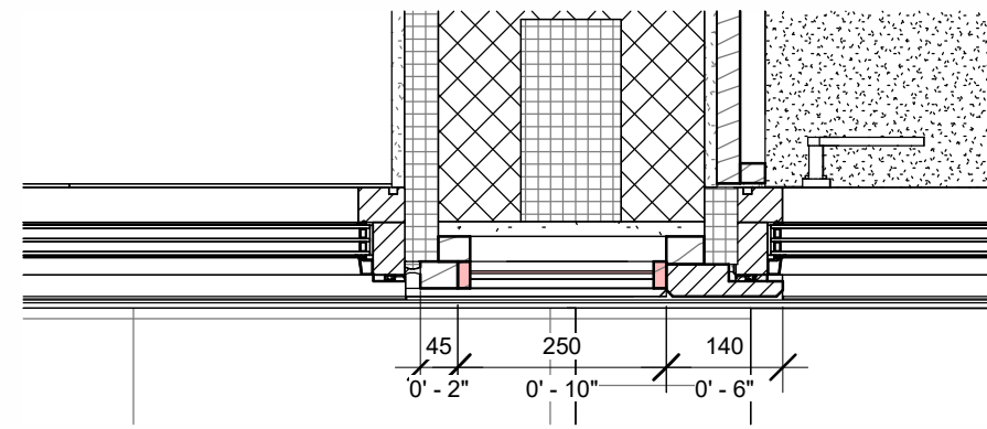
W13 & W17 JAMB DETAILS (UPPER PLAN C)
