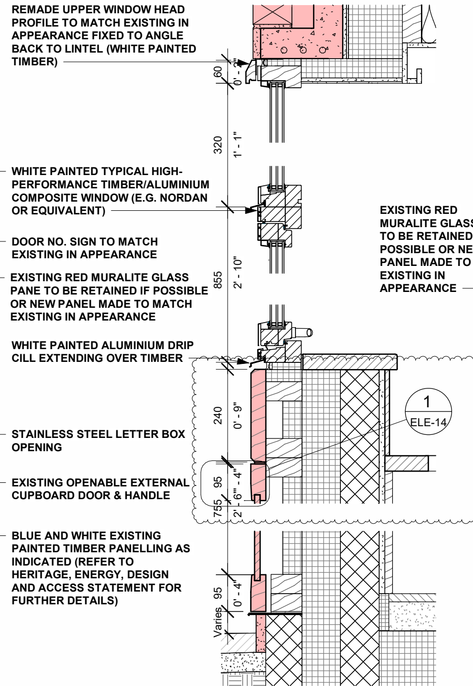
W13 HEAD AND CILL DETAIL (SECTION A) SCALE 1:10
