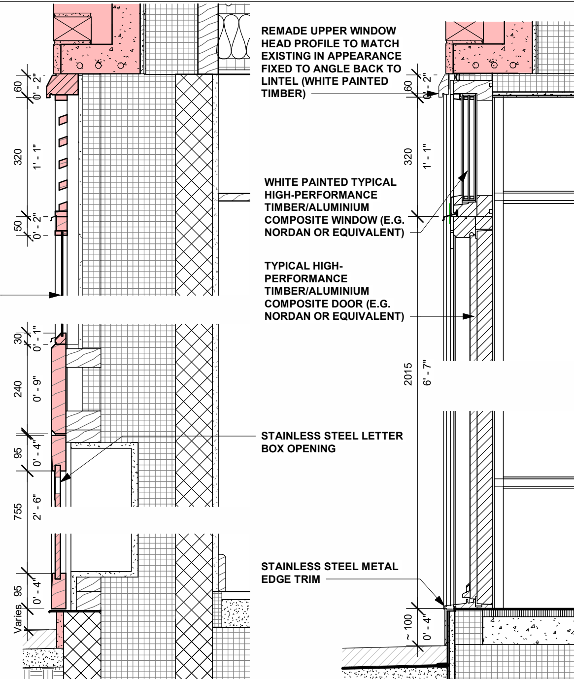
W13 HEAD AND CILL DETAIL (SECTION B) SCALE 1:10
