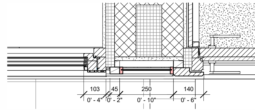
W13 & W17 JAMB DETAILS (MID PLAN B) SCALE 1:10
