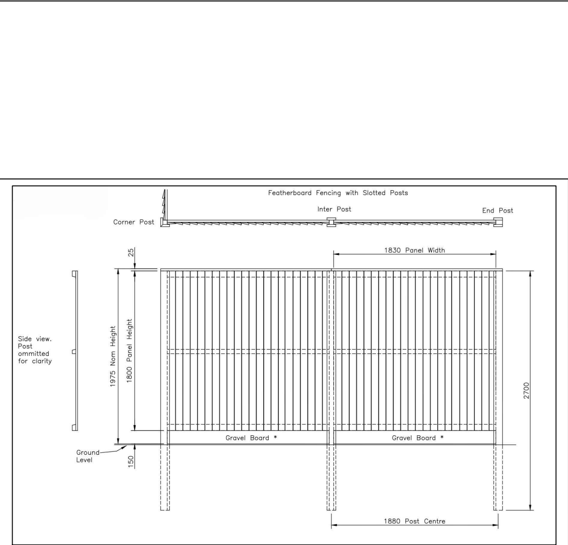
Details for proposed 1.80m high Timber Flat Top Featherboard Fence Panels, as supplied by Jacksons fencing or equivalent. Details to be found on www.jacksons-fencing.co.uk
