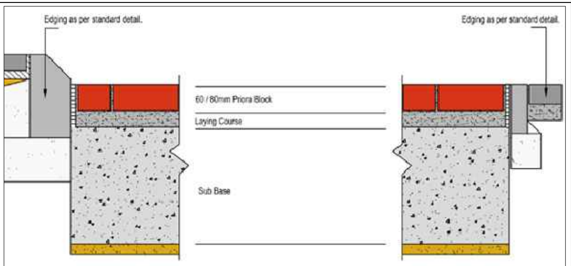
Details for proposed Priora Permeable Block Paving in Charcoal, laid in Herringbone pattern, 200x100x60mm, as supplied by Marshalls Landscaping or equivalent. Details to be found on www.marshalls.co.uk
