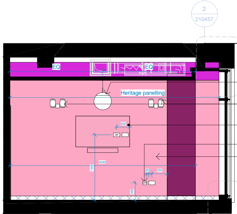
E CC-00-009 - Meeting Room - Elevation East 1 : 50
