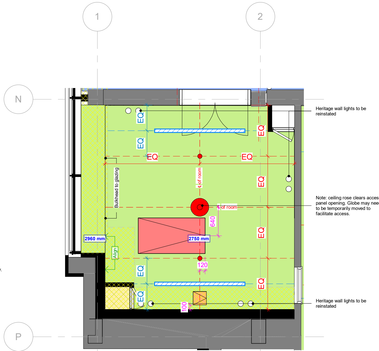
2 CC-00-009 - Meeting Room - Reflected Ceiling Plan 1 : 50
