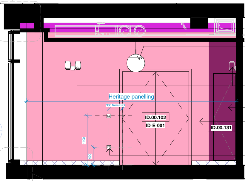
W CC-00-009 - Meeting Room - Elevation West 1 : 50
