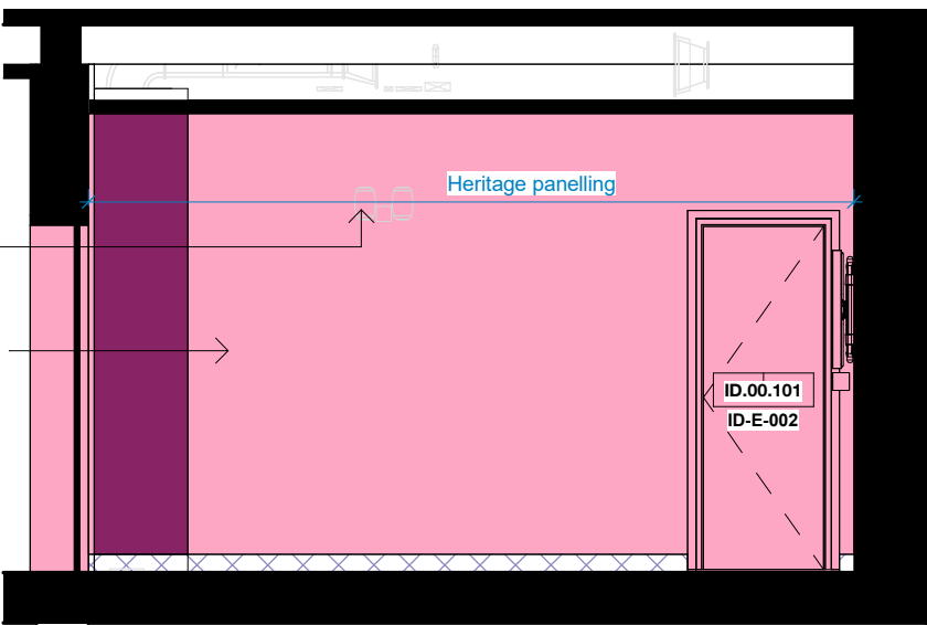
N CC-00-009 - Meeting Room - Elevation North 1 : 50
