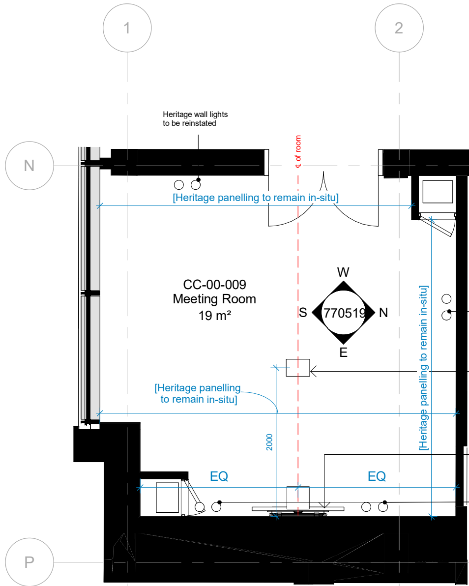
1 CC-00-009 - Meeting Room - Floor Plan 1 : 50
