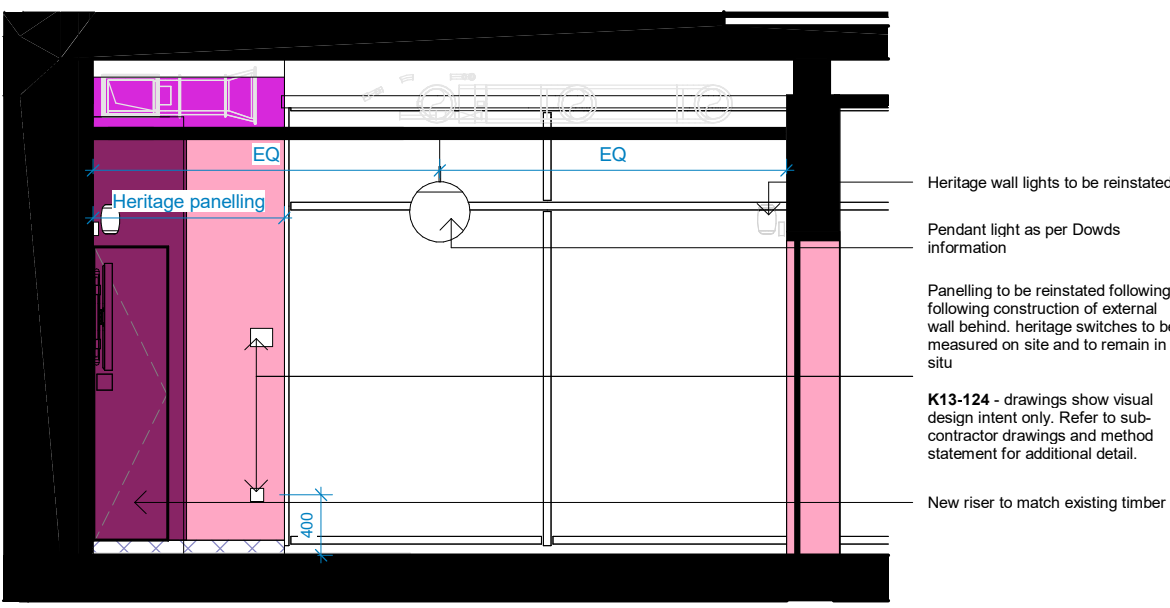
S CC-00-009 - Meeting Room - Elevation South 1 : 50
